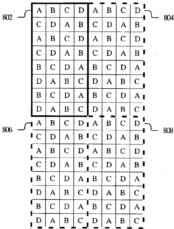
Figure 8A
