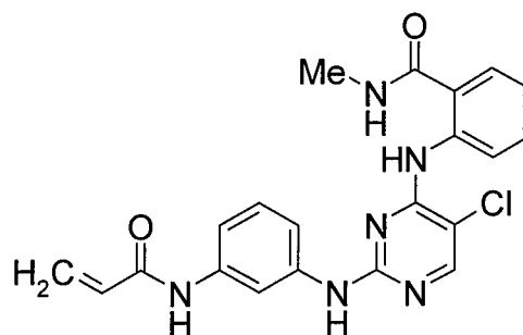
Compound XIII-1
