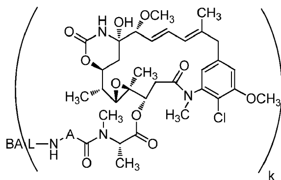
30 (Formula IA)
