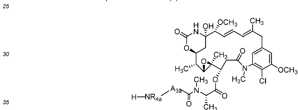
(Formula II)
