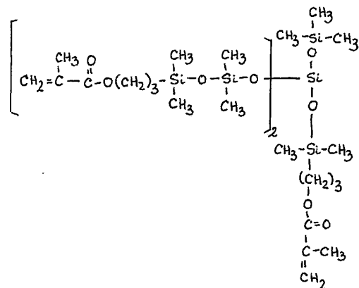
Tris( \gamma -methacryloxy propyl tetramethyl disiloxanyl)trimethyl siloxy silane
