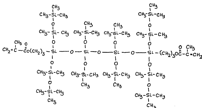
1,7-Bis( p -methacryloxypropyl)-1,1,7,7-tetra(pentamethyl disiloxanyl)-3,3,5,5-tetra(trimethylsiloxy)-tetrasiloxane
