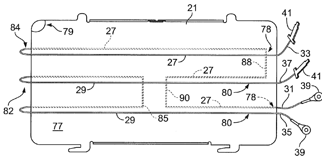
FIG. 4 (Prior Art)
