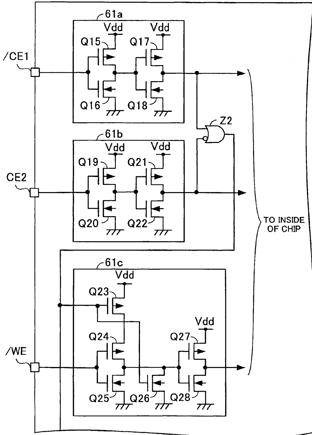
FIG. 8 PRIOR ART
