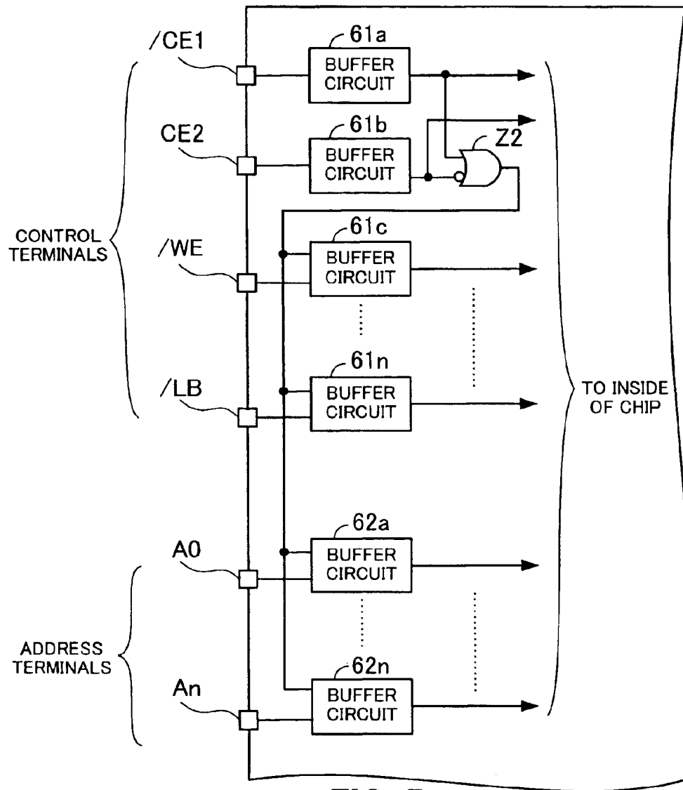
FIG. 7 PRIOR ART
