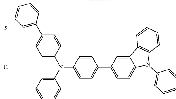
PCBA1BP
