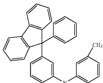
BPAFLP
