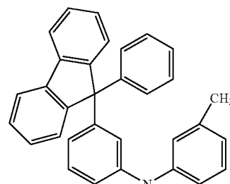
BPAFLP
