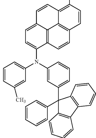
1,6mMemFLPAPrn
