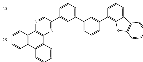
2mDPTBPDBq-11
