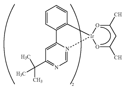
[Ir(tBuppm)_2(acac)]
