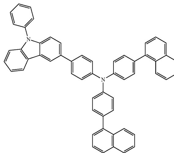
PCBNBB
