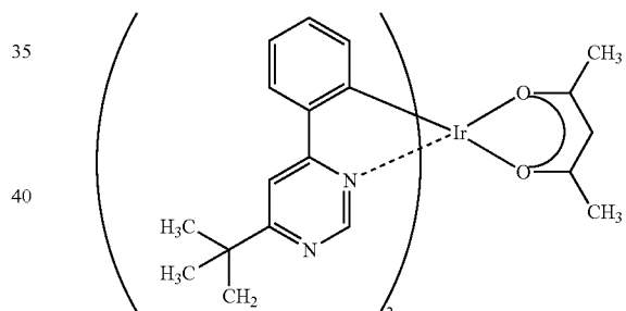
[Ir(tBuppm) 2 (acac)]
