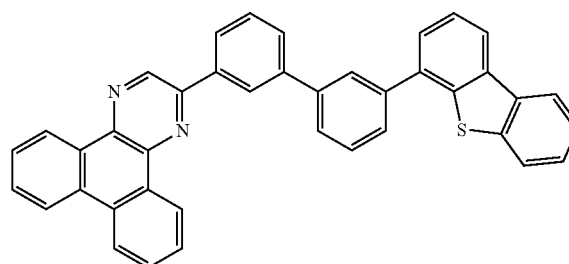
2mDBTBPDBq-II
