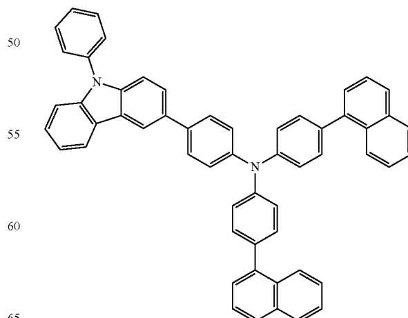
PCBNBB
