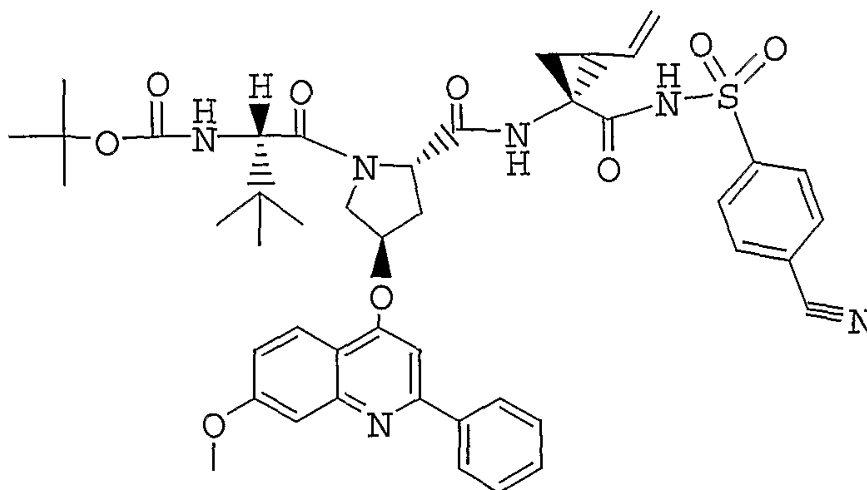
Compound 41
