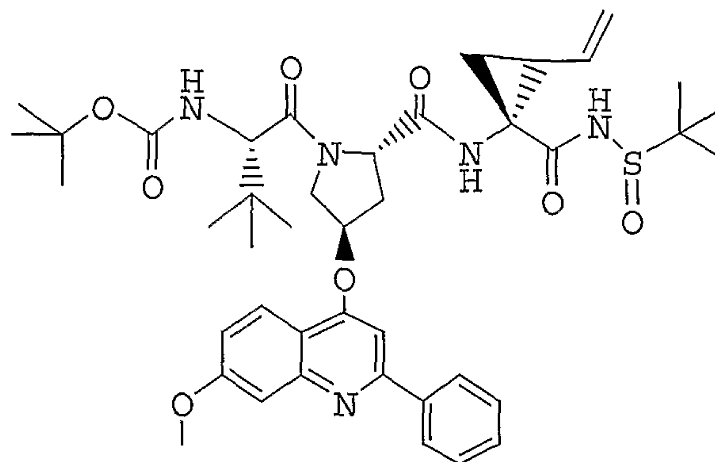
Compound 62
