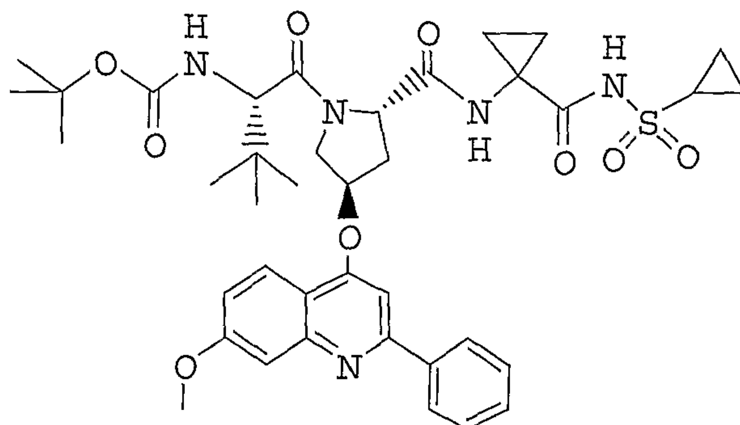
Compound 67
