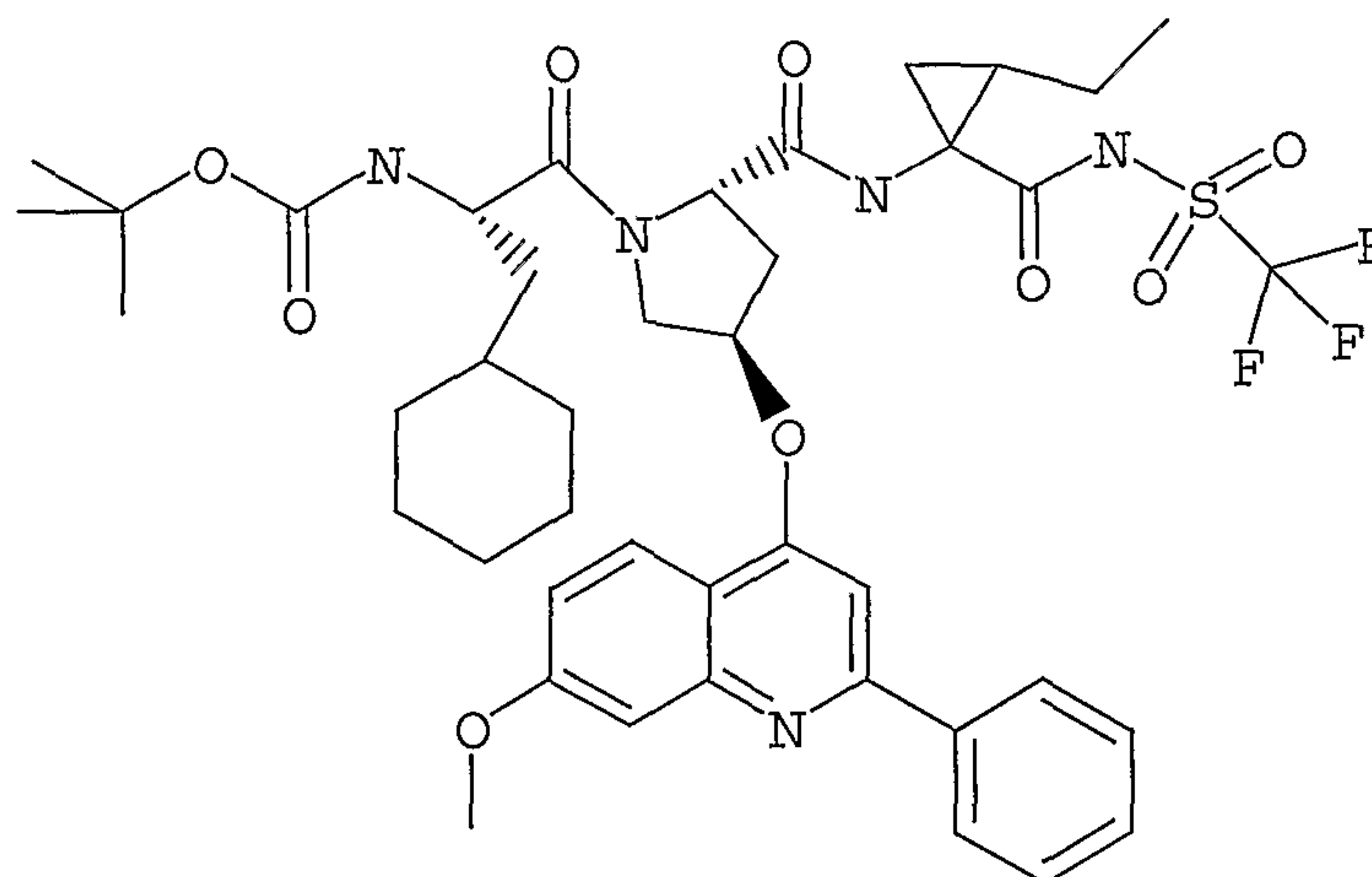
Compound 80
