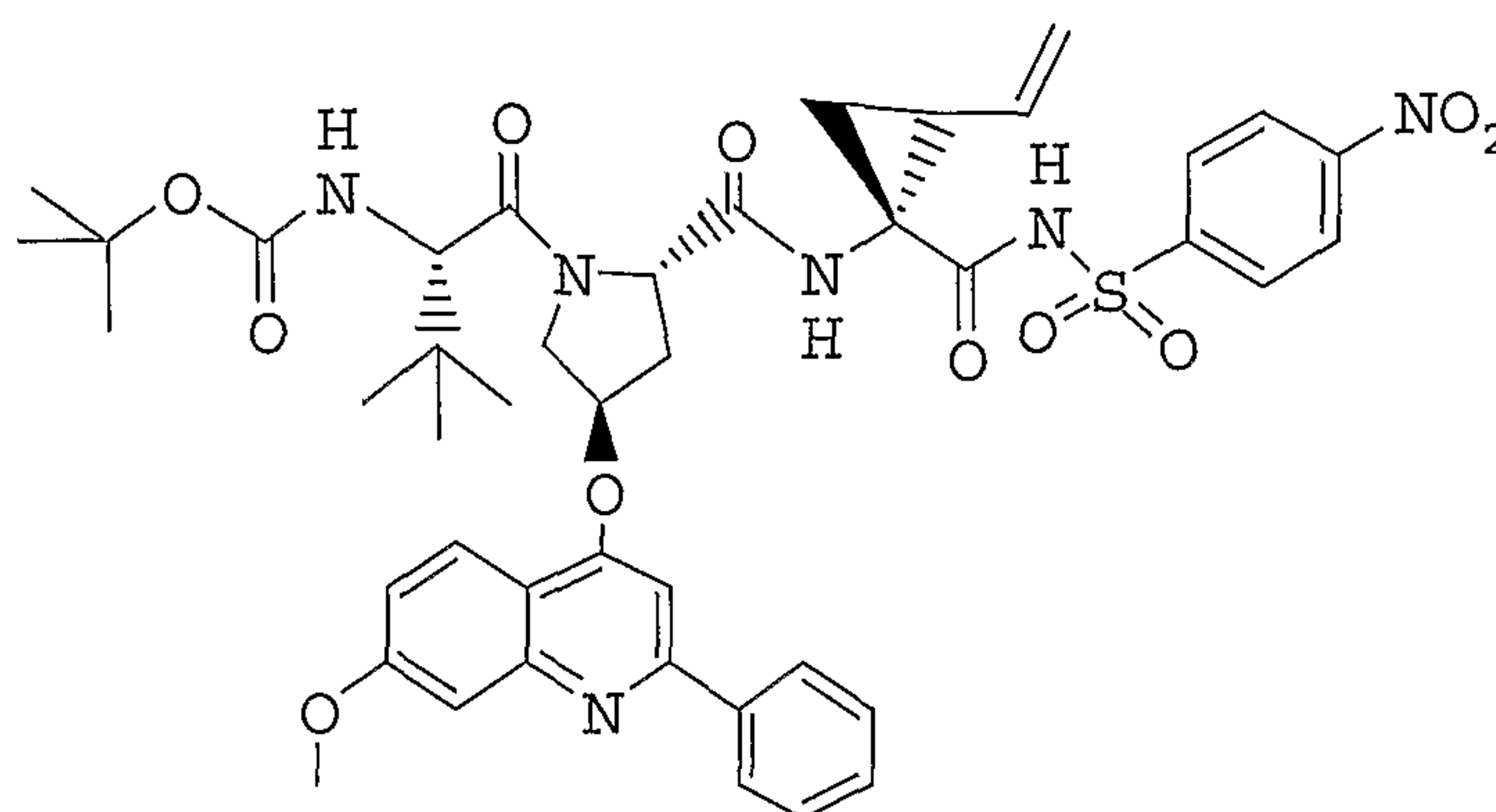
Compound 52
