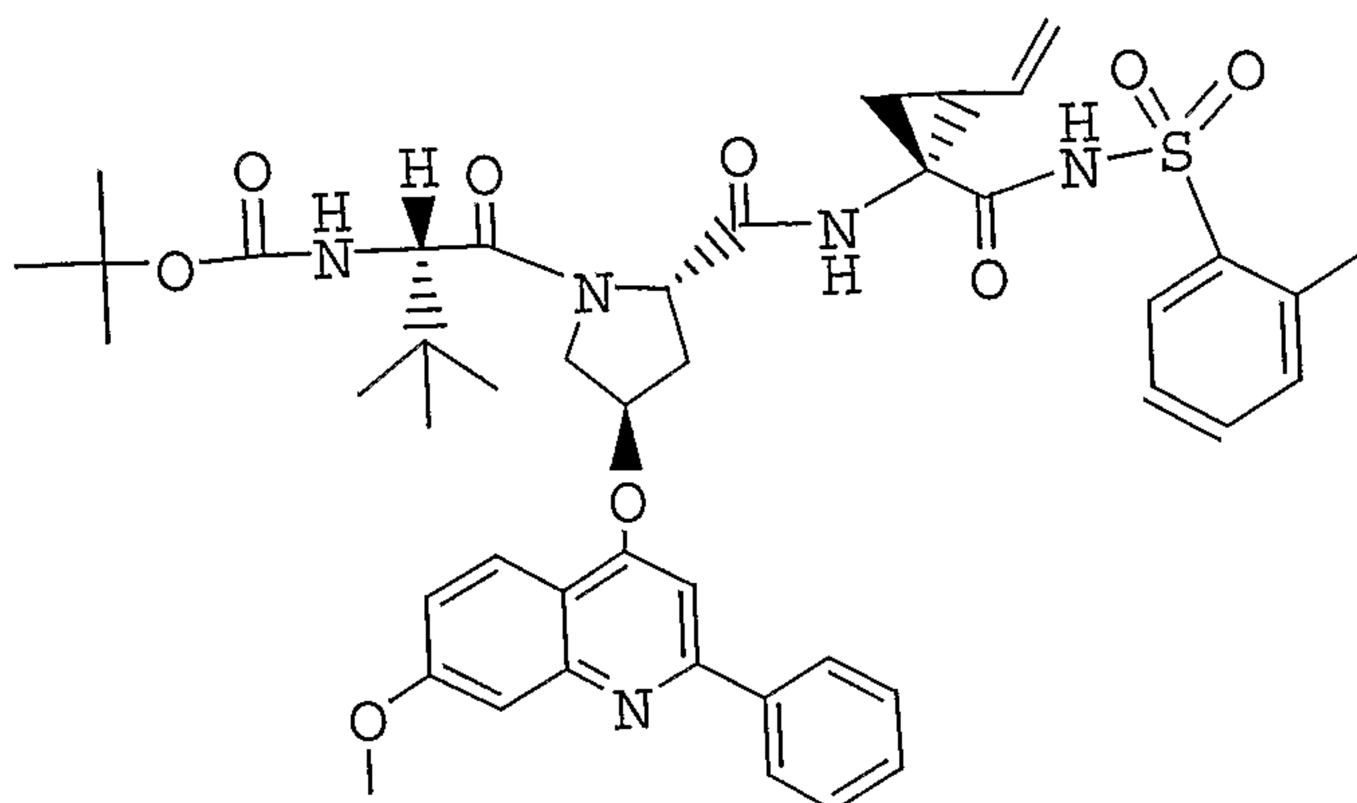
Compound 63
