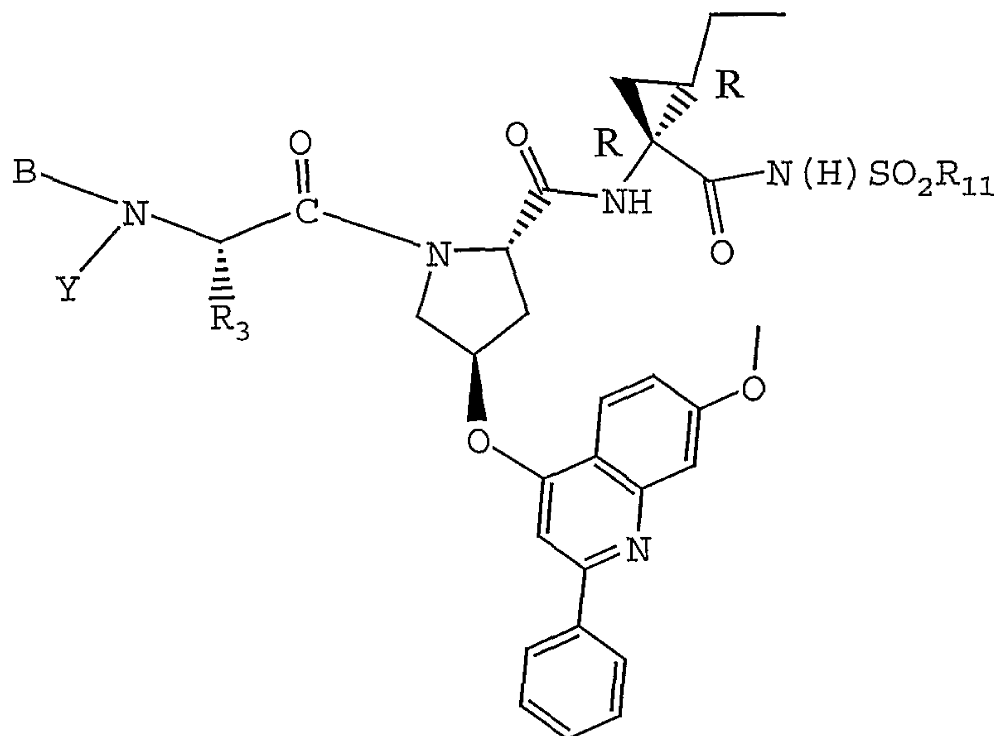
Formula IV
