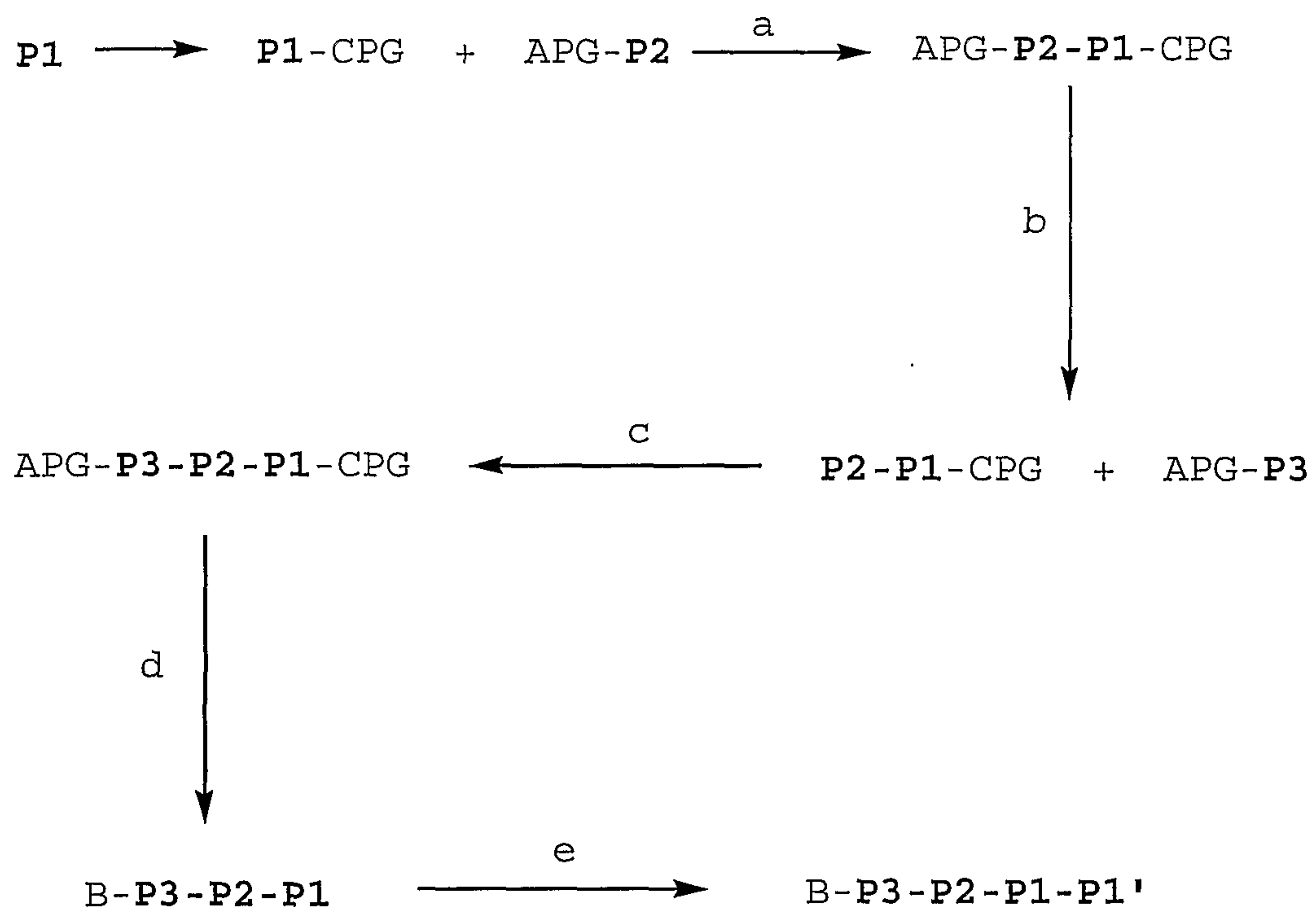
Scheme I
