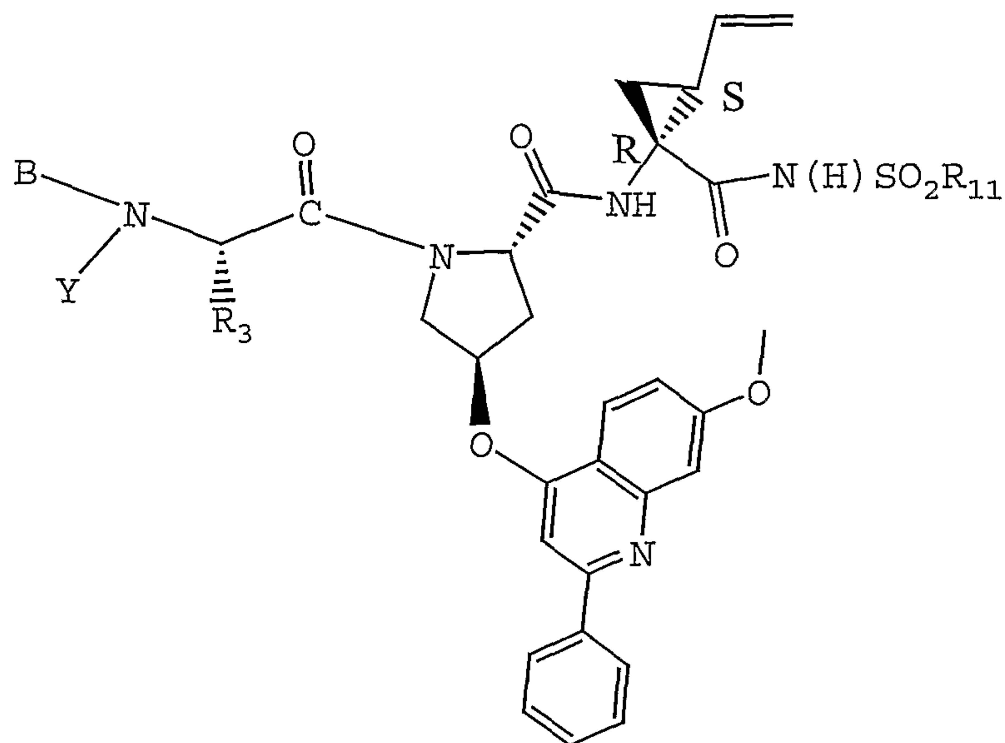
Formula III
