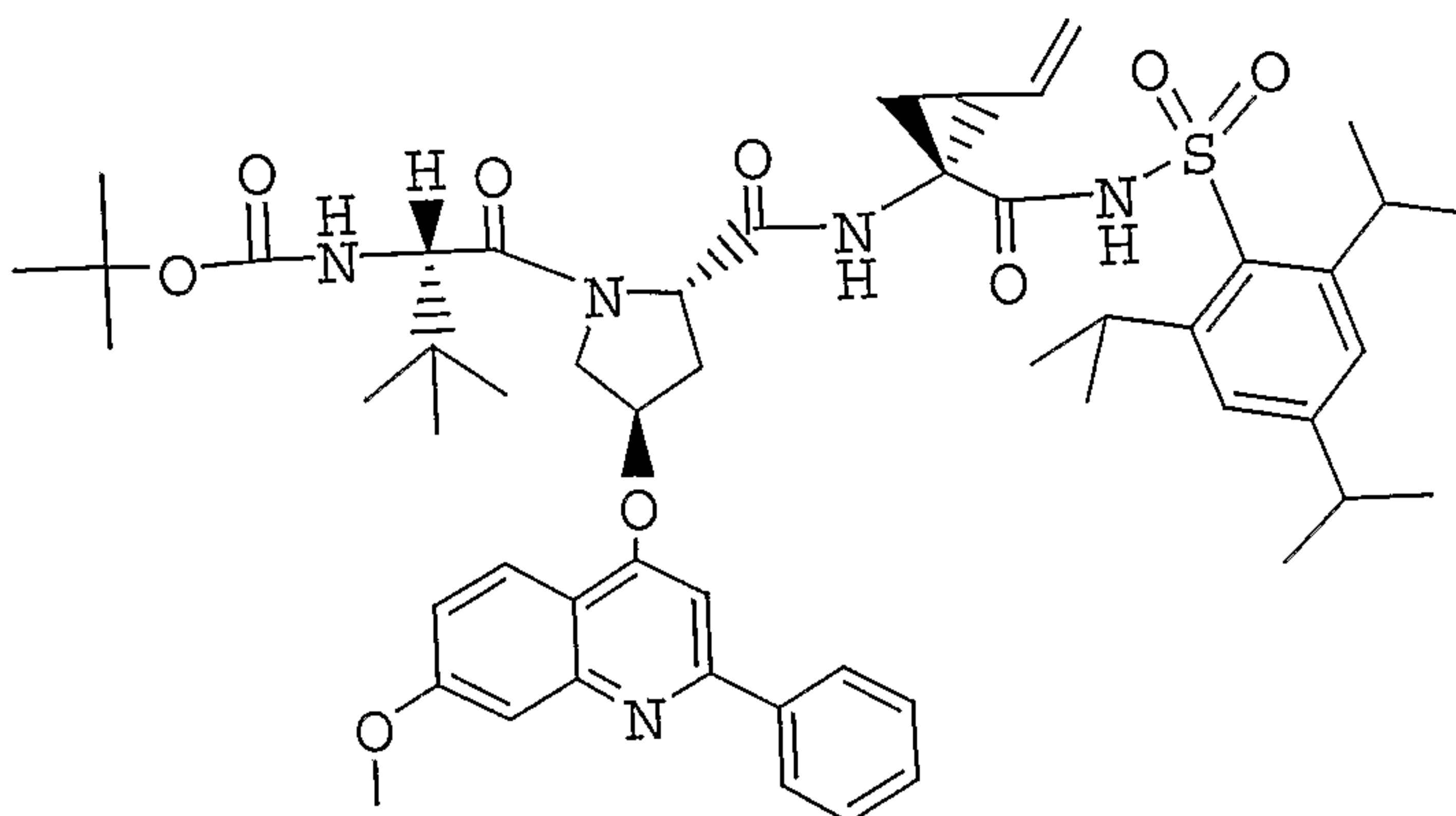
Compound 64
