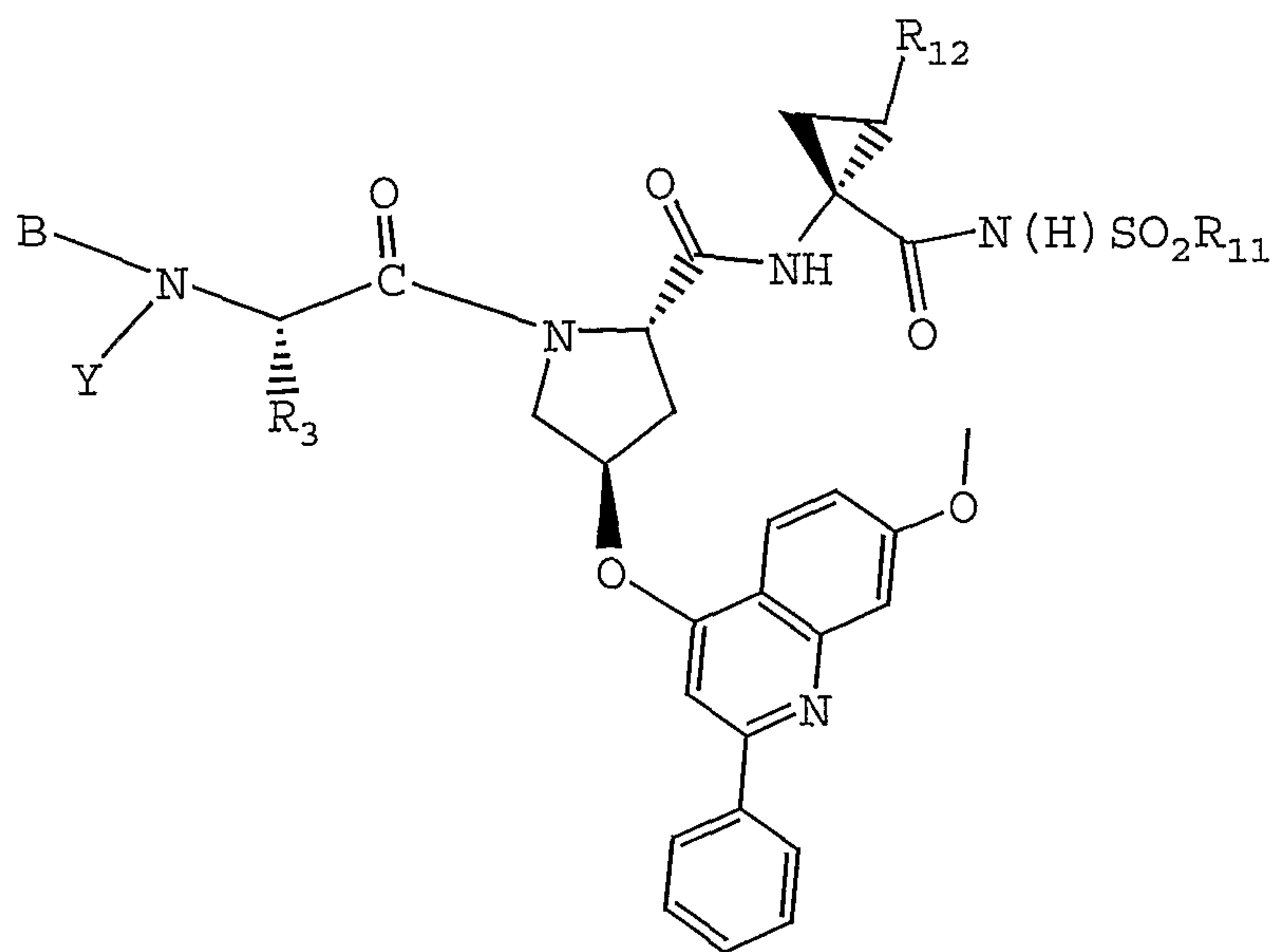
Formula II
