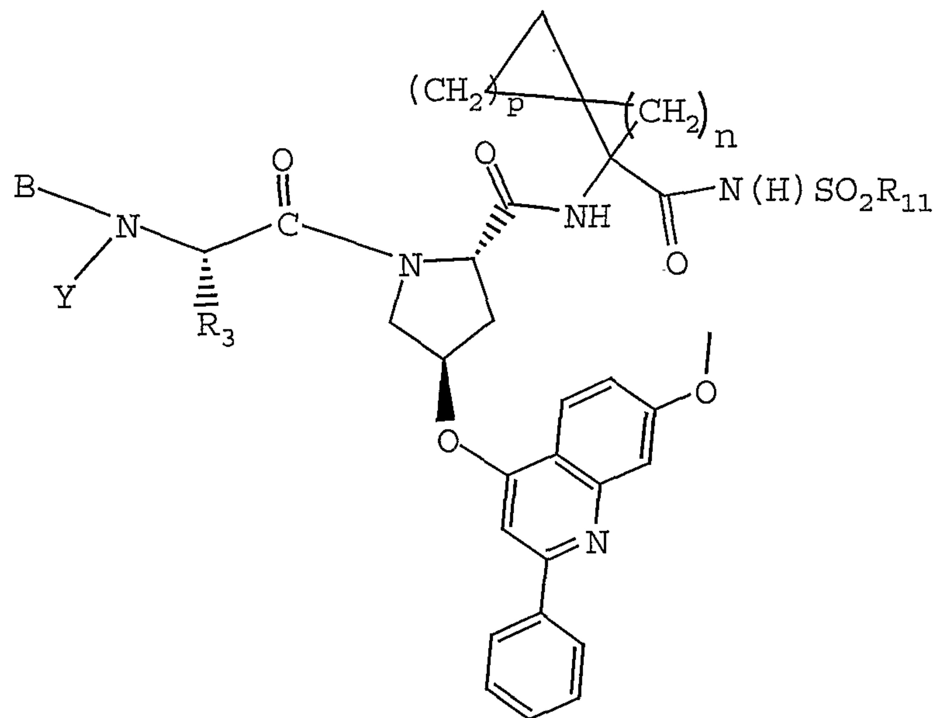
Formula V
