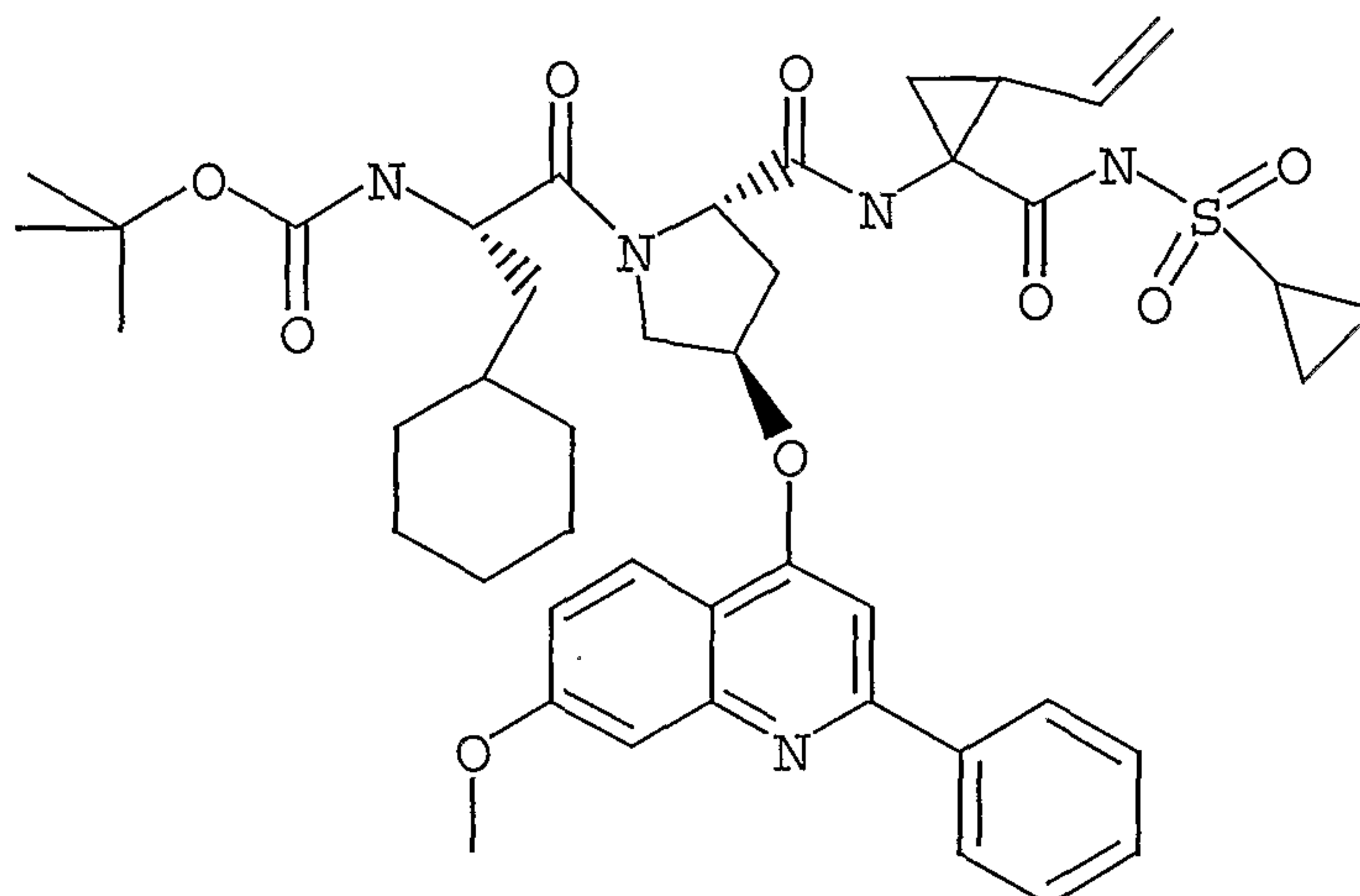
Compound 79
