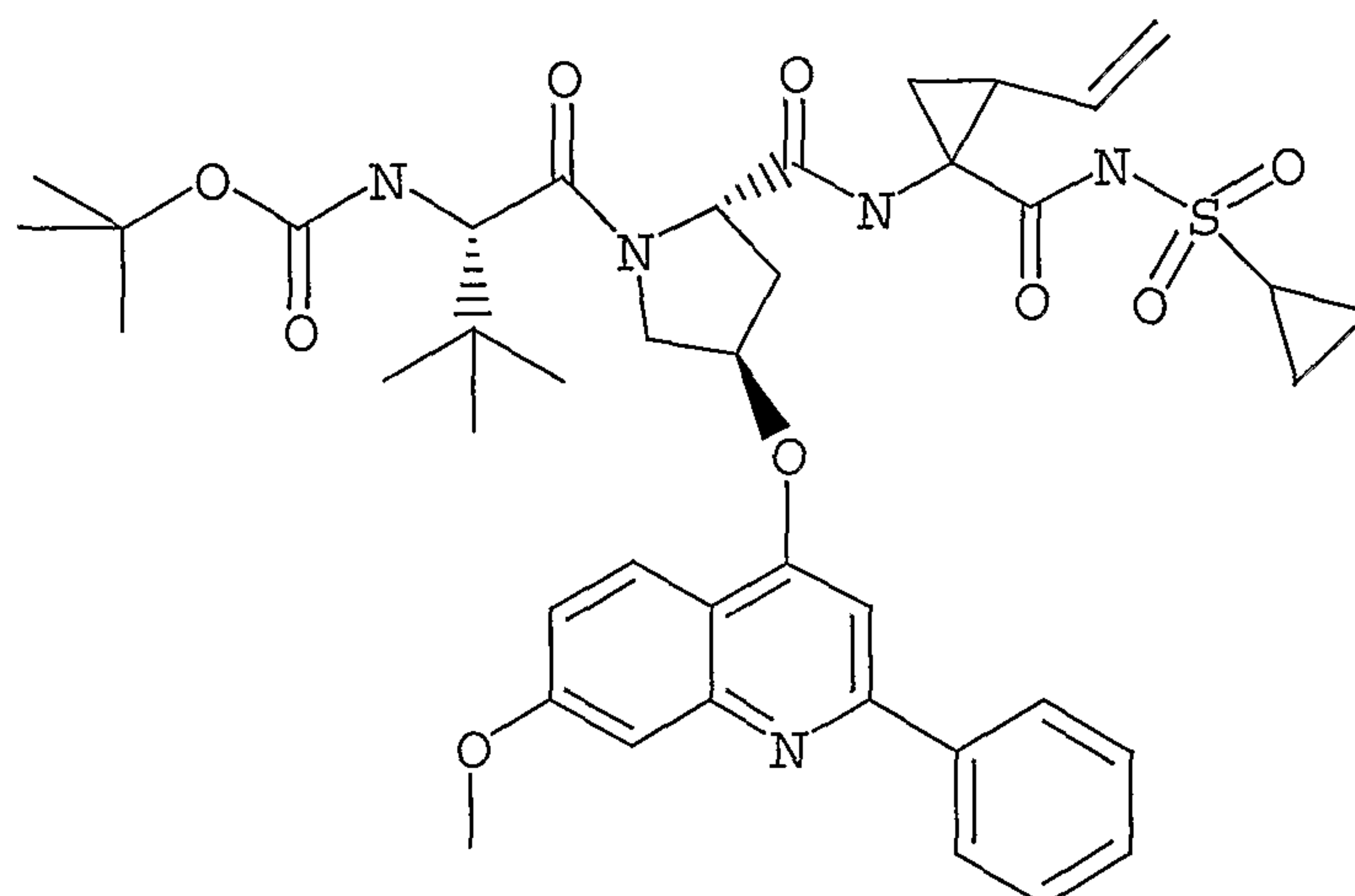
Compound 91
