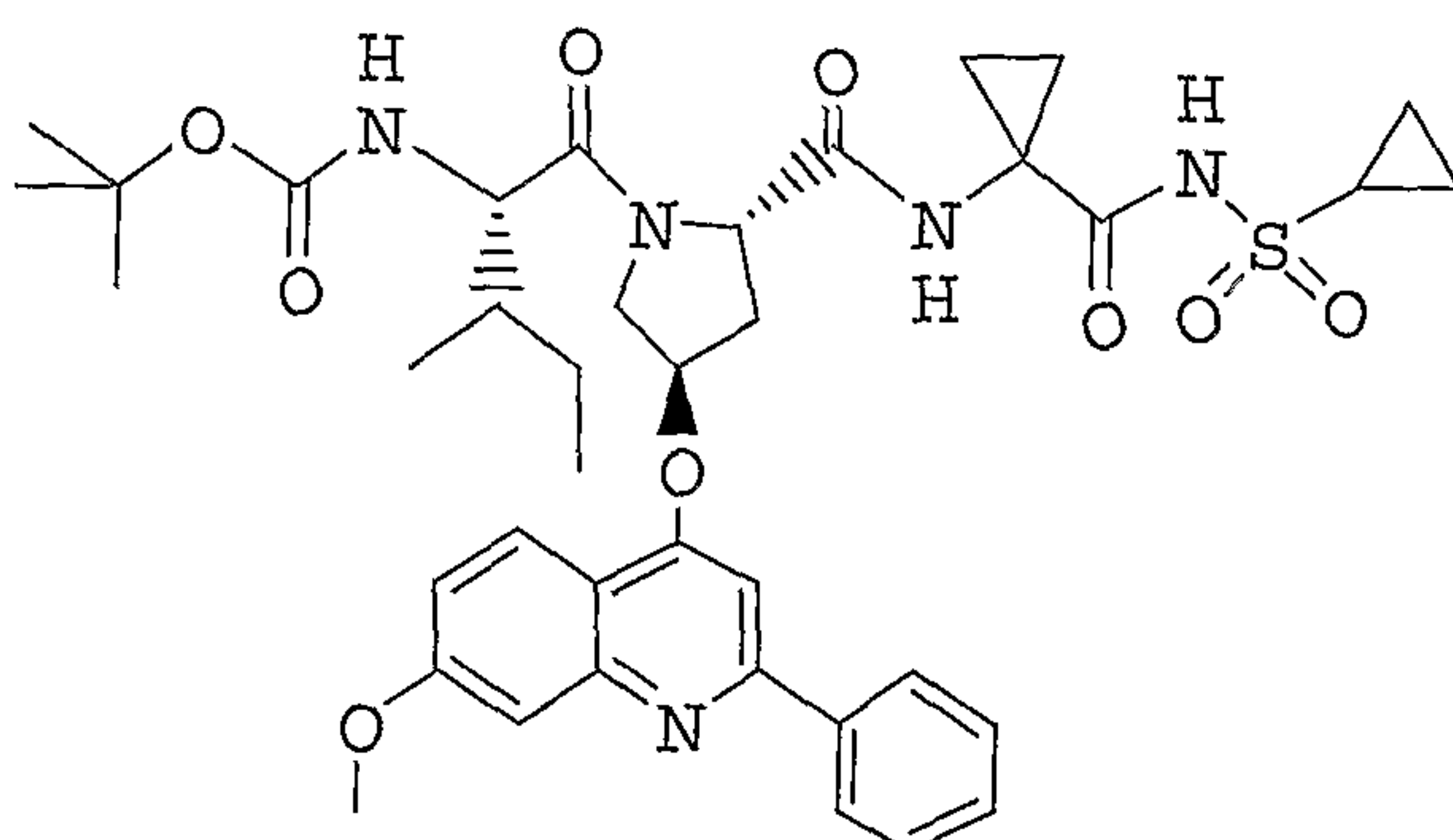
Compound 68
