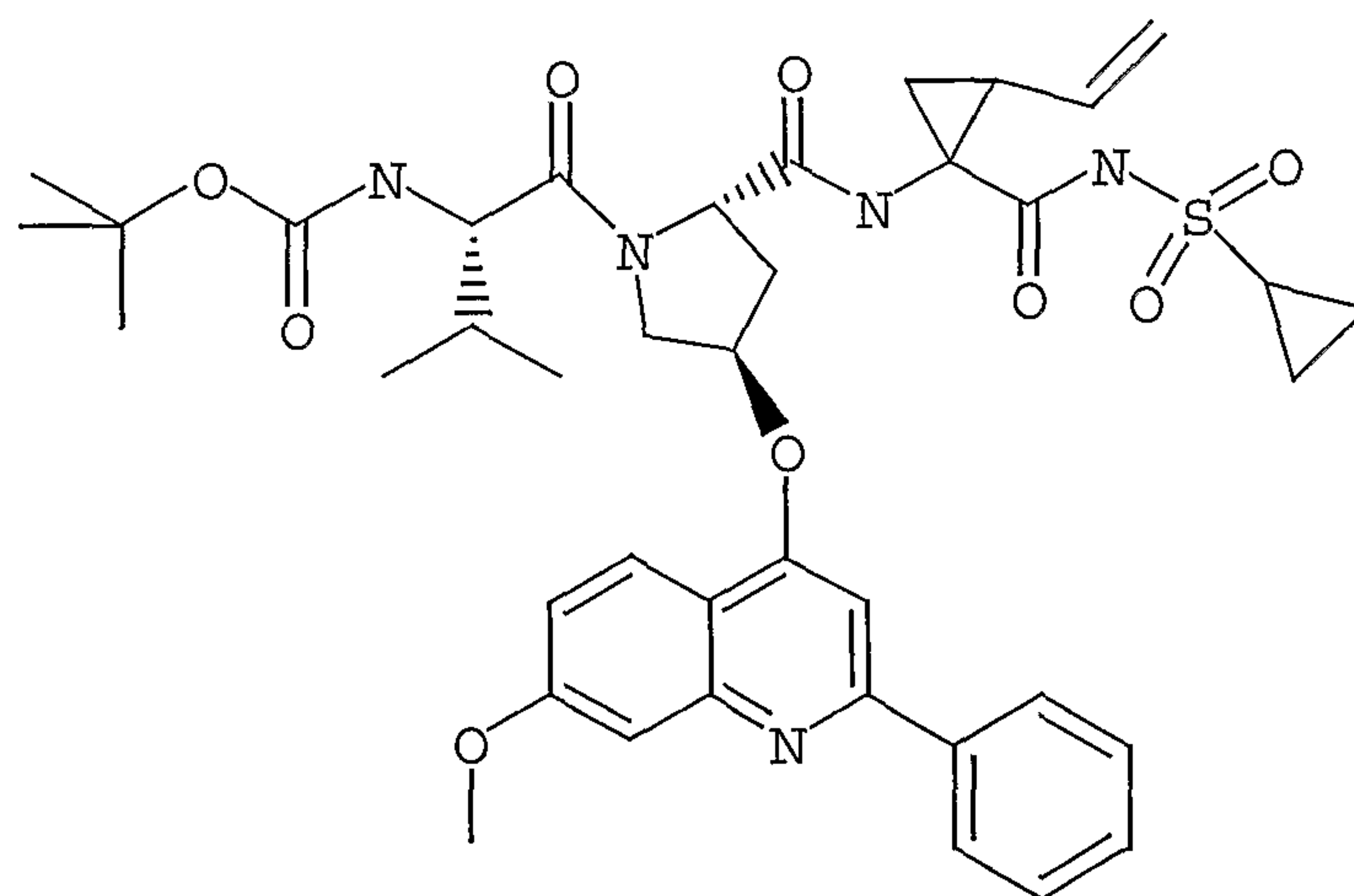
Compound 92
