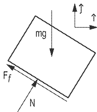
FREE BODY DIAGRAM OF JUST THE BLOCK
