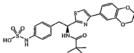
4-((S)-2-(4-(2,3-Dihydrobenzo[b][1,4]dioxin-6-yl)thiazol-2-yl)-2-pivalamidoethyl)phenylsulfamic acid
