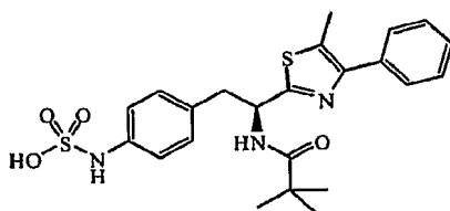
(S)-4-(2-(5-Methyl-4-phenylthiazol-2-yl)-2-pivalamidoethyl)phenylsulfamic acid
