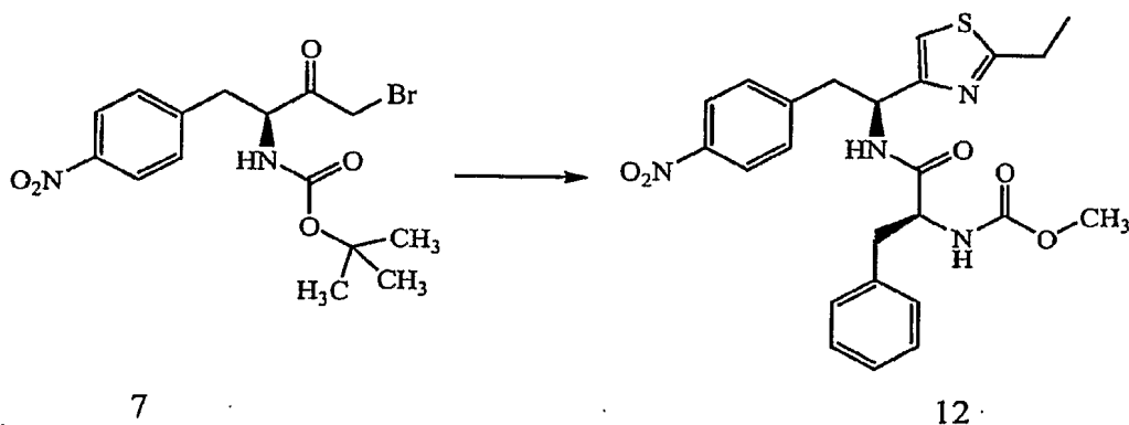
Scheme IV
