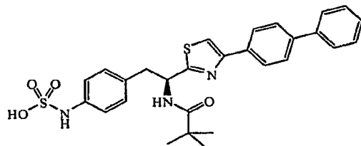
(S)-4-(2-(4-(Biphen-4-yl)thiazol-2-yl)-2-pivalamidoethyl)phenylsulfamic acid
