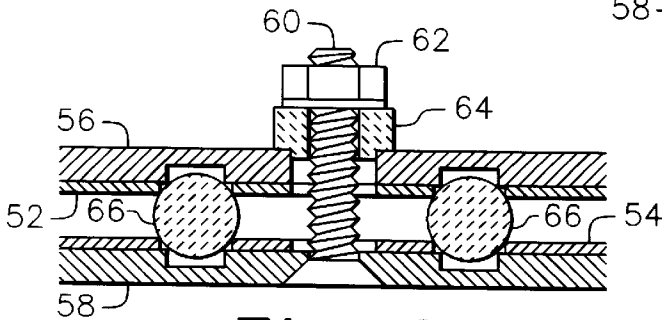
Fig. 6 (PRIOR ART)
