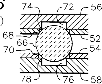
Fig. 7 (PRIOR ART)
