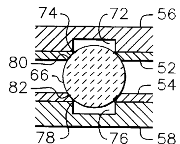
Fig. 8 (PRIOR ART)
