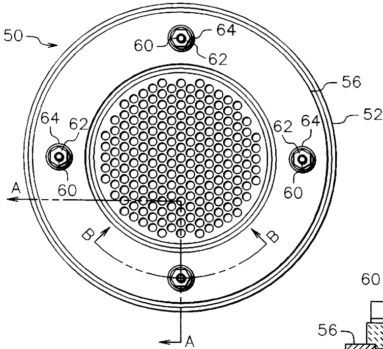
Fig. 4 (PRIOR ART)
