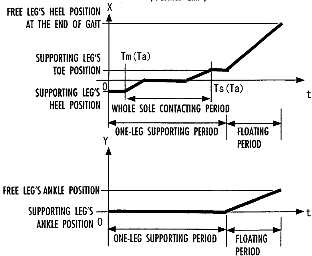
FIG.7 ( DESIRED ZMP )
