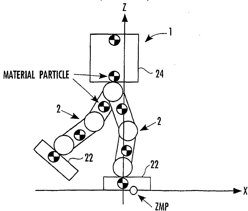
FIG.11 ( FULL MODEL )
