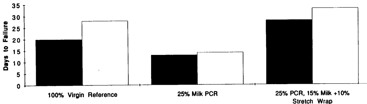
Fig. 1 Environmental Stress Crack Resistance 32 oz. Nonhandle, Square Base
