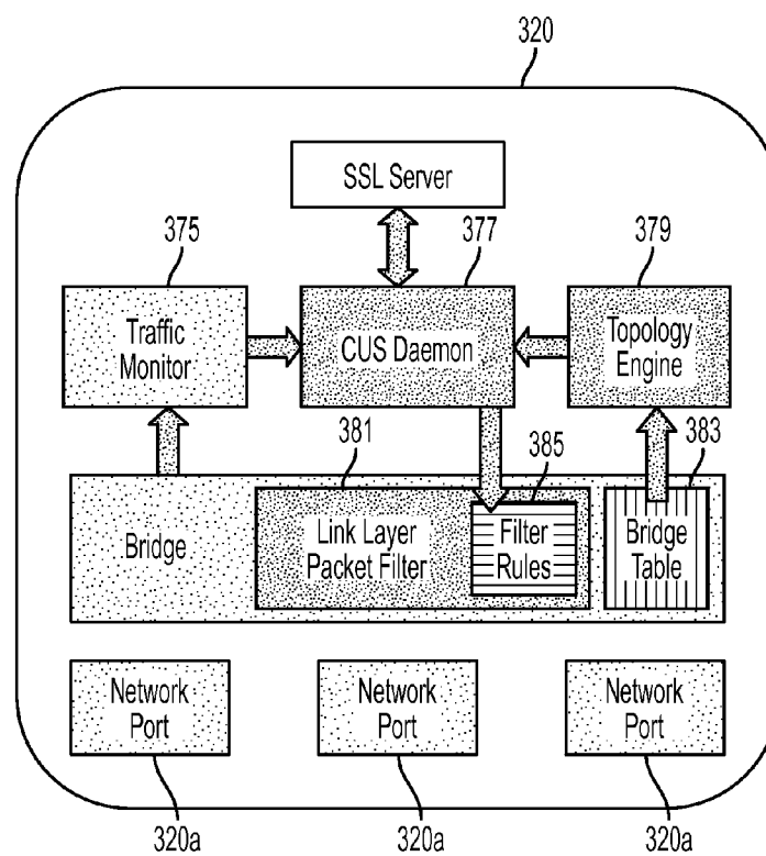
Software modules in a CUS Switch
