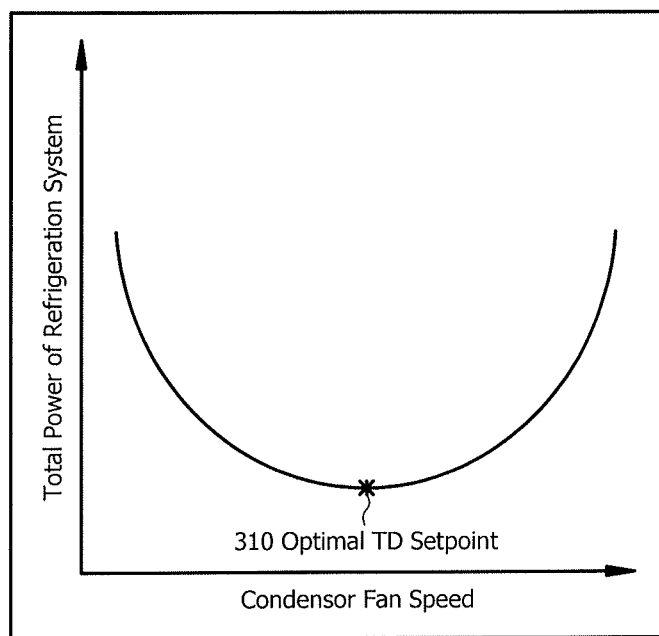
FIG. 3D
