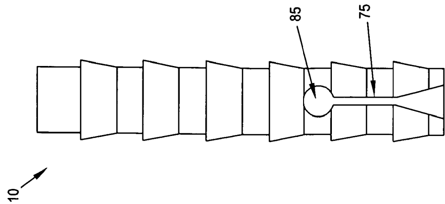
FIG. 45 SLIT THROUGH ONE SIDE PLUS MATERIAL BARB
