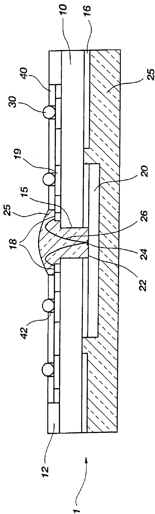
Fig. 2 (PRIOR ART)
