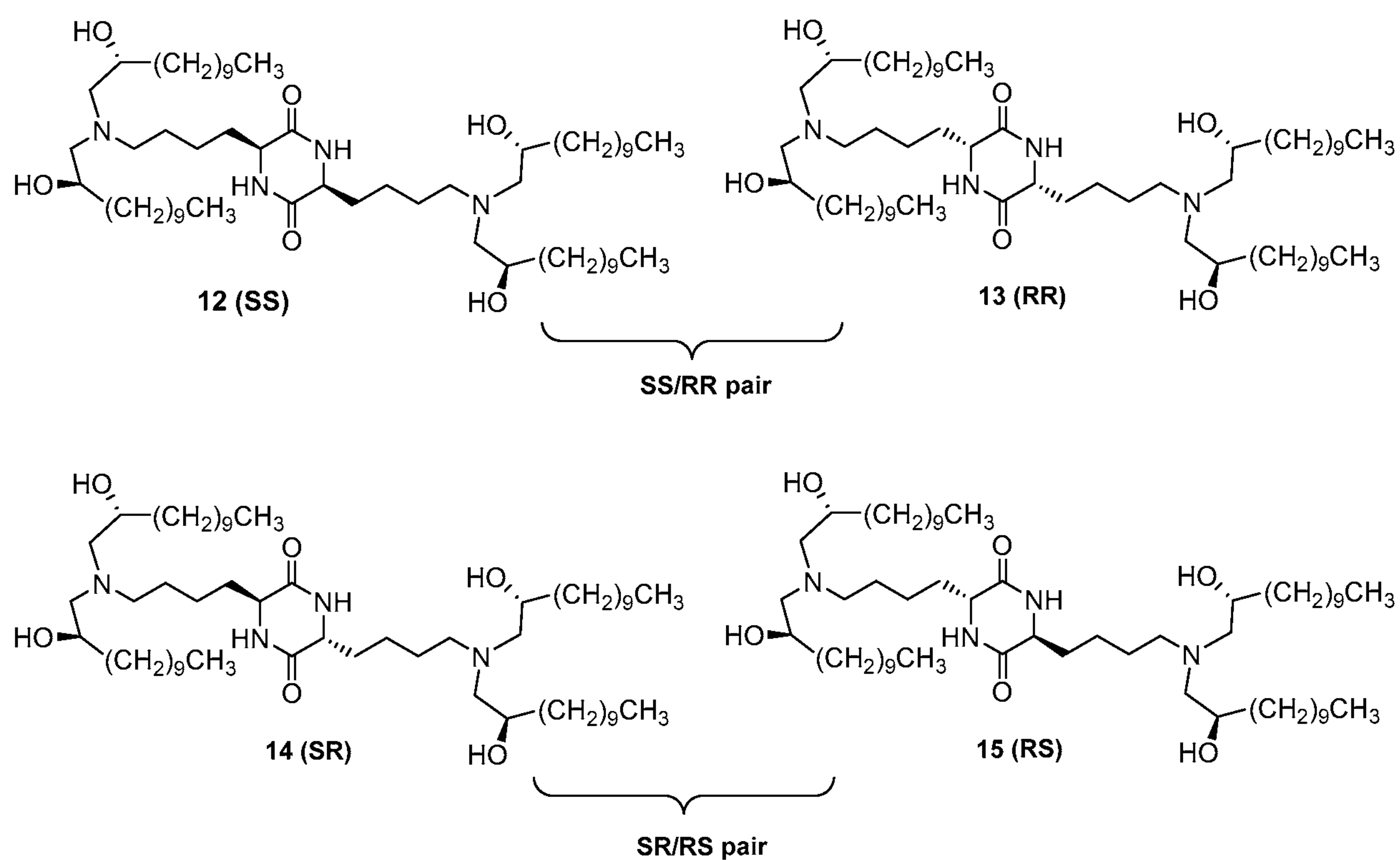
Scheme 3. Chiral compounds 12-15.
