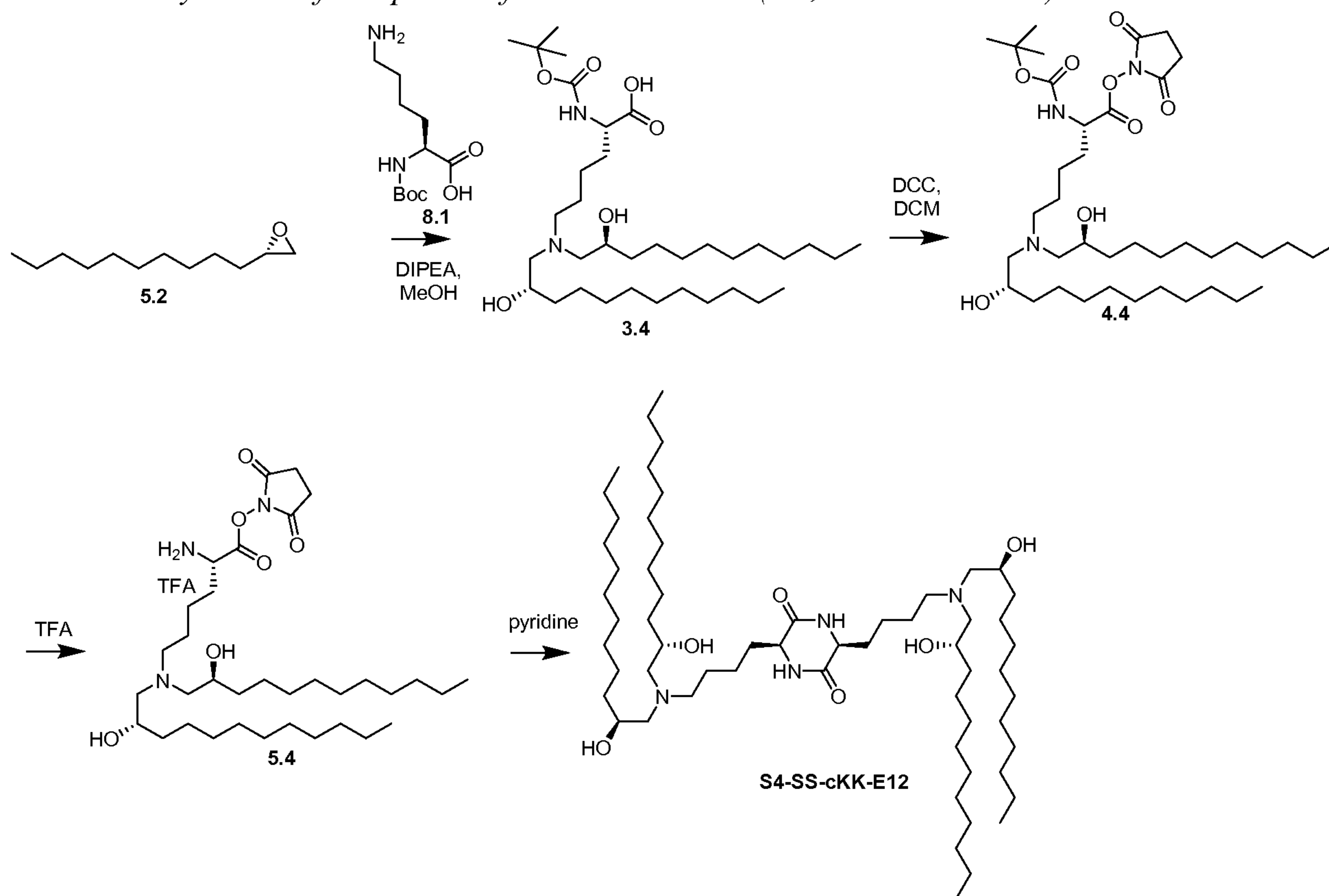
Scheme 7: Synthesis of compound of Formula I.b.1.ii (i.e., S4-SS-cKK-E12)
