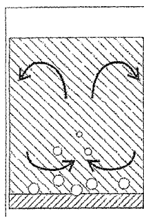
Quiet boiling
