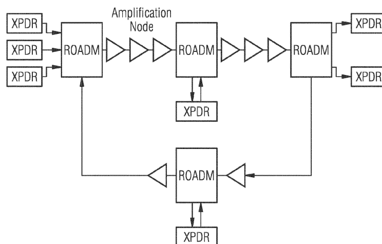
ROADM node with pass-through and add/drop traffic
