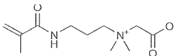
1-(carboxylatomethyl)-1-methyl-4-(2-methylprop-2-enoyl)piperazin-1-ium (CK 1585):
