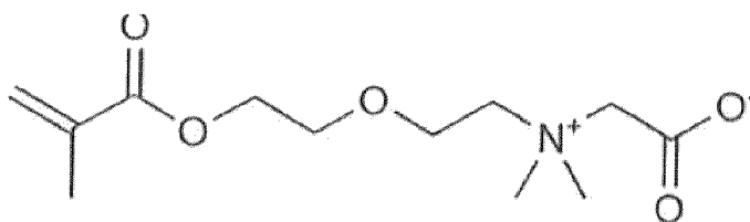
2-{dimethyl[3-(2-methylprop-2-enamido)propyl]-azaniumyl}acetate (CK 1588):
