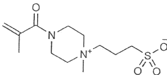
3-[dimethyl(2-{2-[(2-methylprop-2-enoyl)oxy]ethoxy}ethyl)azaniumyl]propane-1-sulfonate (CK1582):
