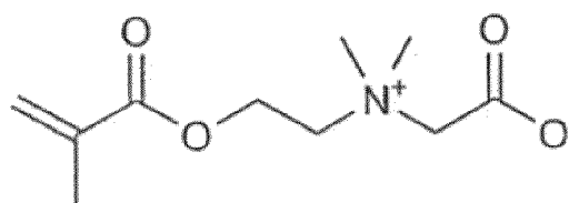
2-[dimethyl(2-{2-[(2-methylprop-2-enoyl)oxy]ethoxy}-ethyl)azaniumyl]acetate (CK 1589):
