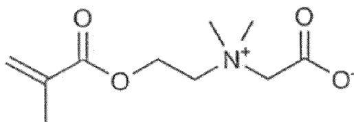
2-[dimethyl(2-{2-[(2-methylprop-2-enyl)oxy]ethoxy}-ethyl)azaniumyl]acetate (CK 1589):
