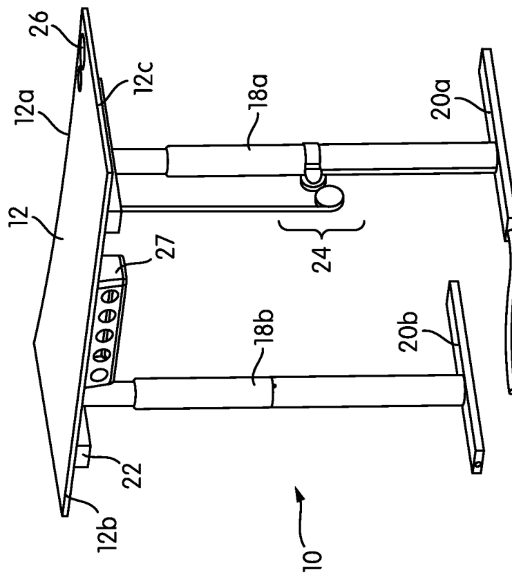
FIG. 5 PRIOR ART
