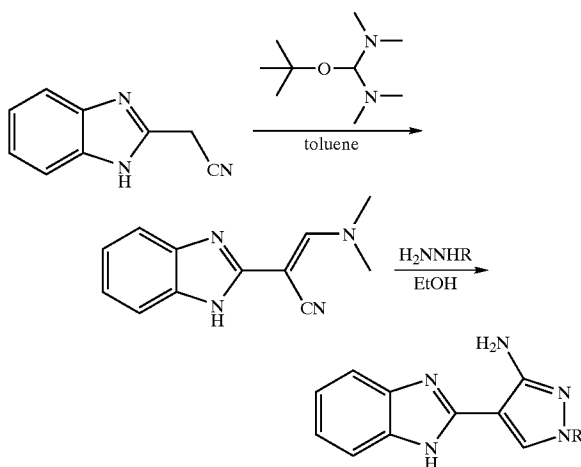
Scheme XVIII: General procedure for the preparation of 2-[3(5)-amino]imidazol-4-yl benzimidazole derivatives
