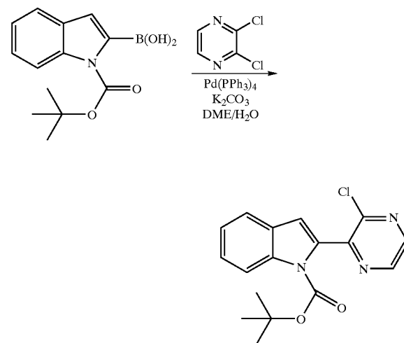
Scheme XIX:
