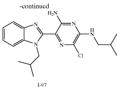
Scheme XV:
