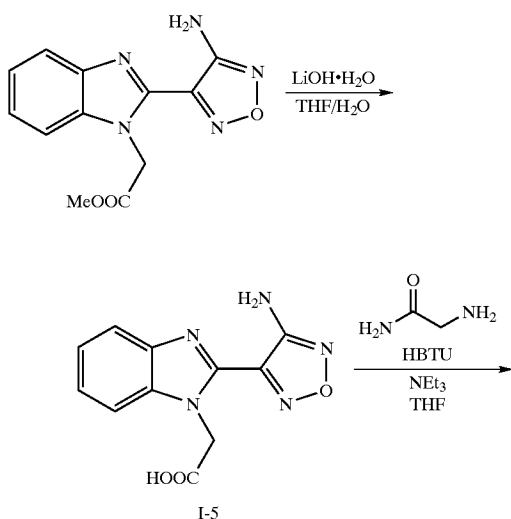
Scheme VI: Preparation of benzimidazole derivative (I-123)
