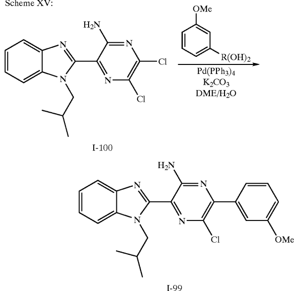
Scheme XV:
