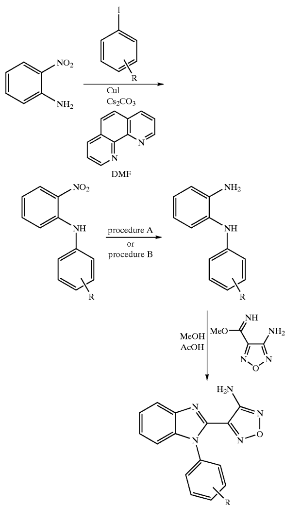
Scheme XII: General procedure for the preparation of 2-(4-amino-1,2,5-oxadiazol-3-yl)-N-aryl benzimidazoles
