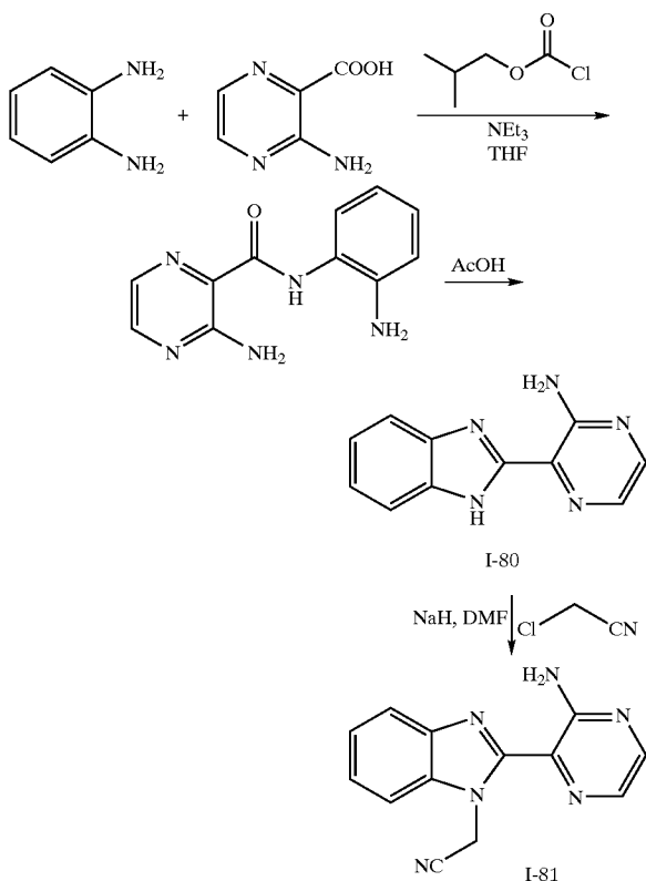
Scheme III: Preparation of 1-cyanomethyl-2-[(3-amino)-2-pyrazinyl]benzimidazole
