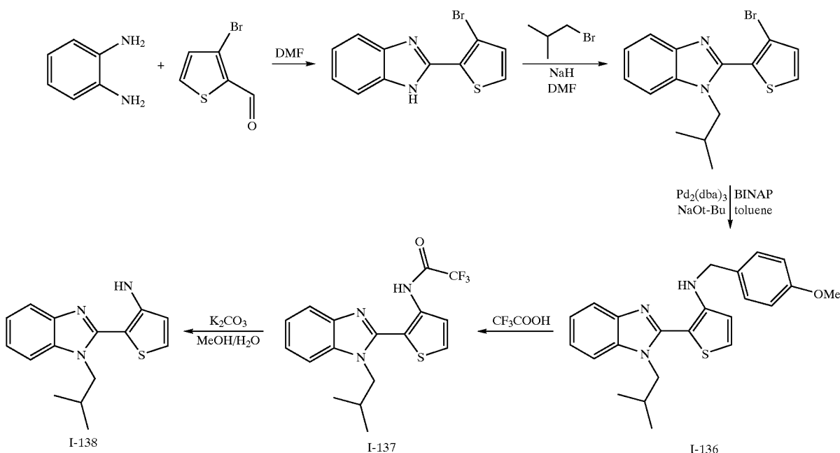
Preparation of 2-(3-Bromo-thiophen-2-yl)-1H-benzimidazole
