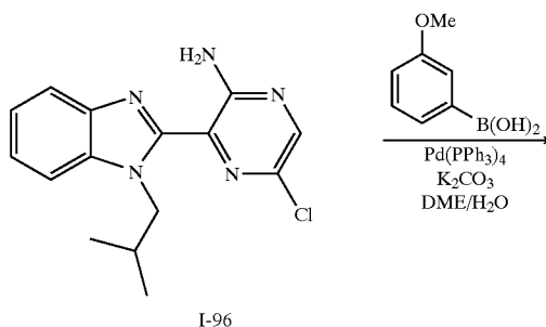
Scheme XVI:
