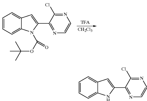
Scheme XX:
