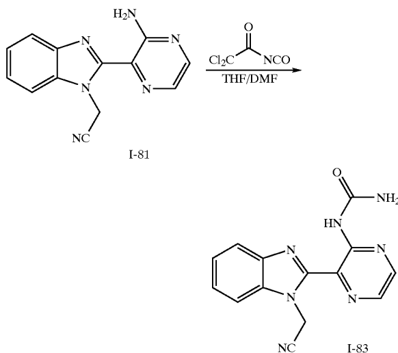
Scheme XXV:
