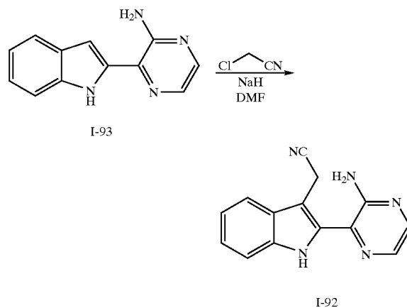
Scheme XXI:
