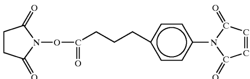
N-hydroxysuccinimide ester maleic function SMPB succinimidyl 4-(p-maleimidophenyl)butyrate
