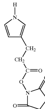
Functionalised PYRROLE in 3' by a succinimide ester.
