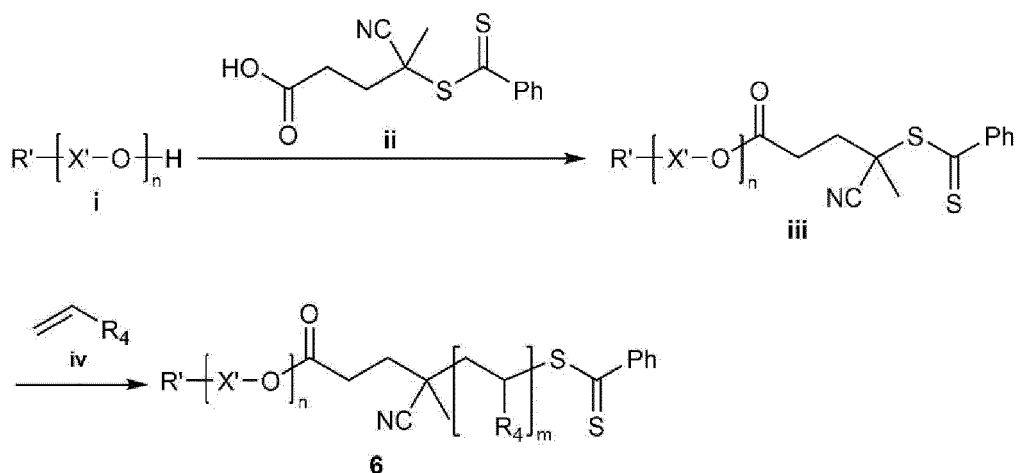
[Reaction Scheme 1]
