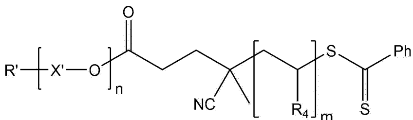
[Chemical Formula 6]
