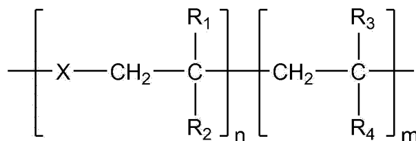
[Chemical Formula 3]
