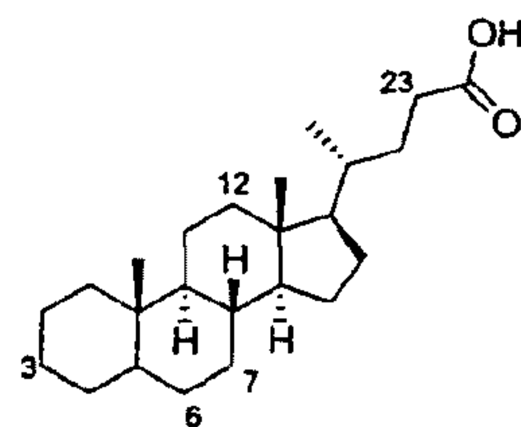
cholanic acid
