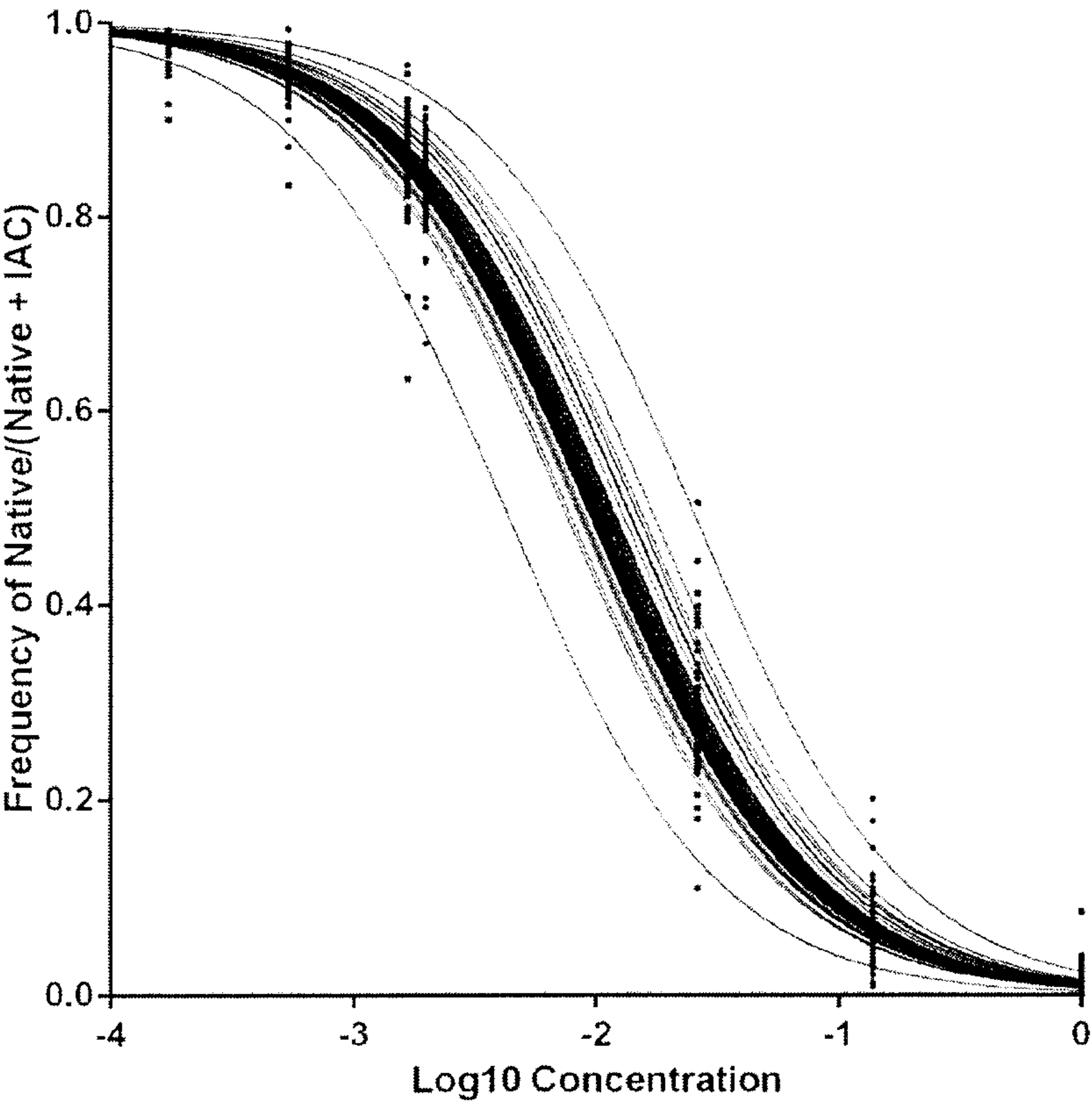
Titration of gDNA in 119 Standardized qNGS assays (SEQC Reagents)
