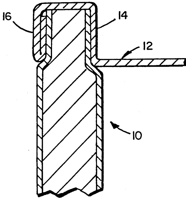
Fig. 1 PRIOR ART
