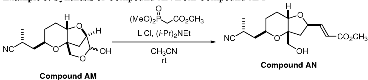
Scheme 18
