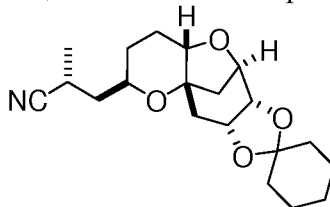
Compound AD,
