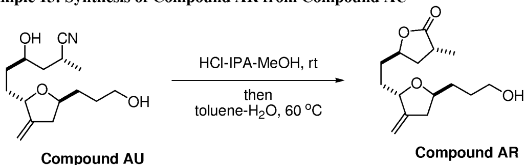
Scheme 23
