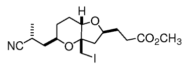
Compound AF
