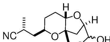
Compound AM
