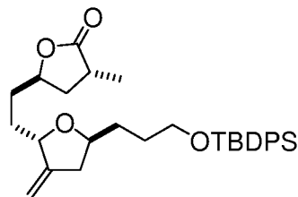
Compound AH
