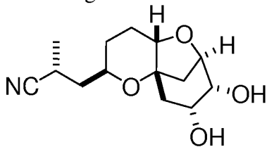
Compound AJ
