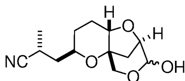
Compound AM,
