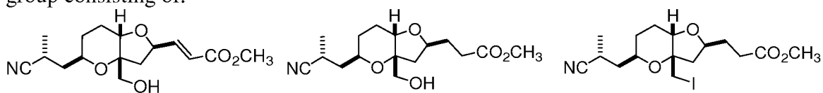
Compound AO
