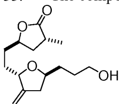
Compound AR
