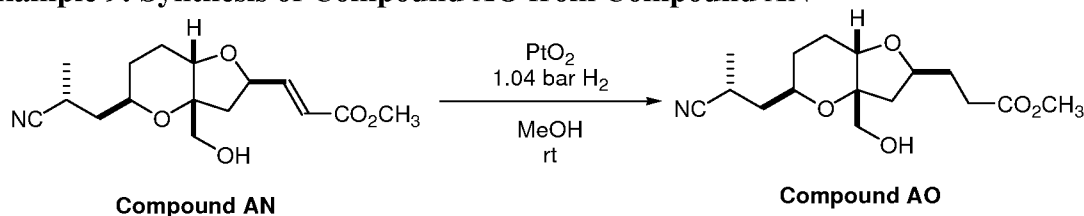
Scheme 19
