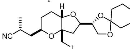
Compound AQ
