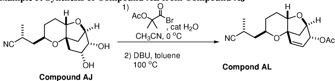
Scheme 15
