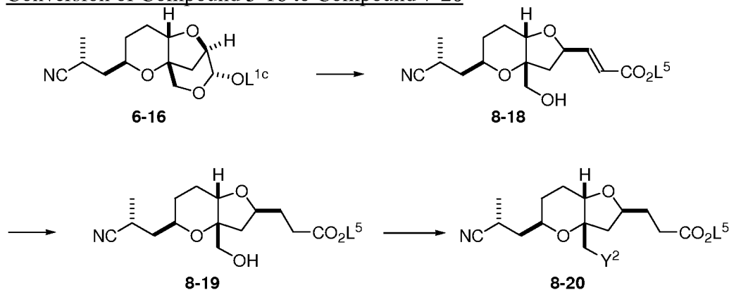
Scheme 8
