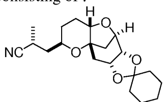
Compound AD
