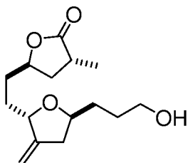
Compound AR
