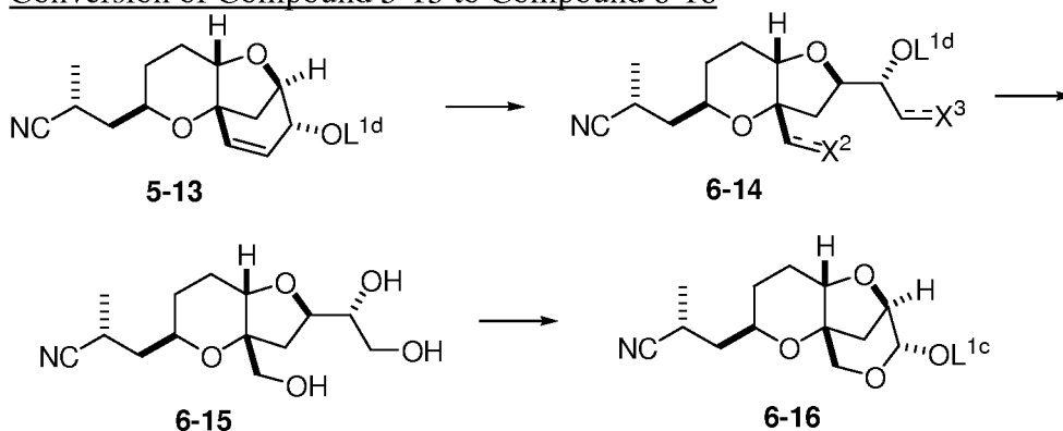
Scheme 6
