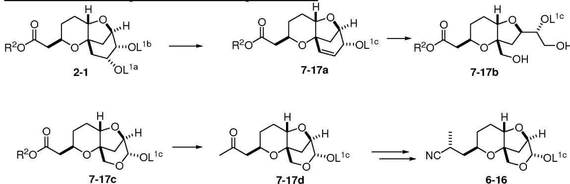
Scheme 7
