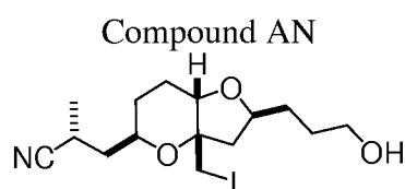
Compound AN
