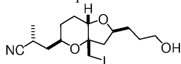
Compound AN
