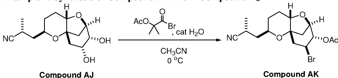
Scheme 14
