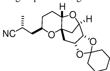
Compound AD
