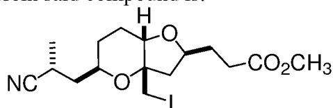
Compound AF,
