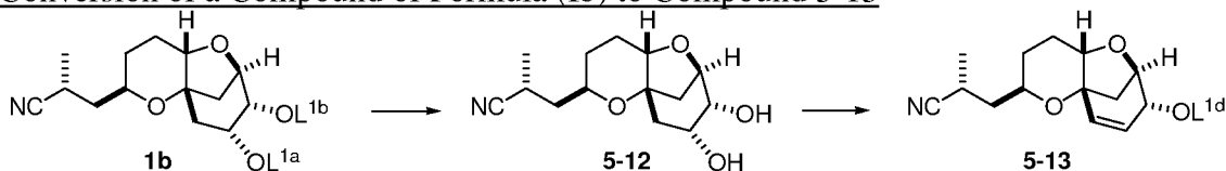
Scheme 5
