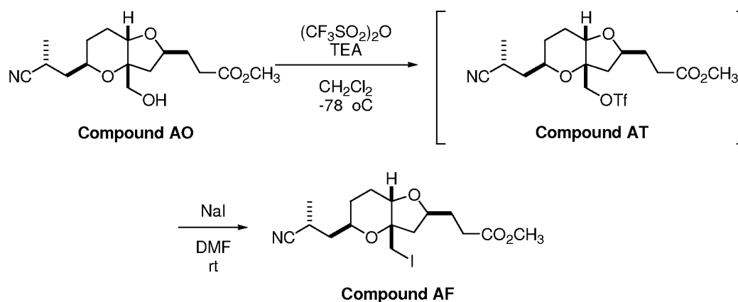
Scheme 20
