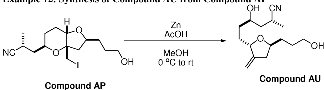
Scheme 22
