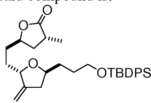
Compound AH
