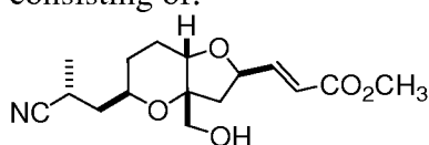
Compound AN
