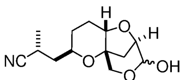
Compound AM.
