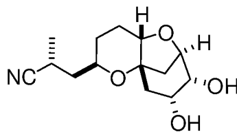
Compound AJ
