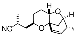
Compound AL
