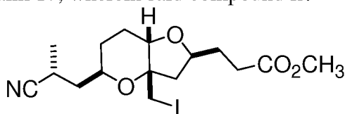
Compound AF,
