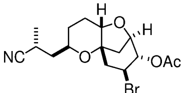
Compound AK
