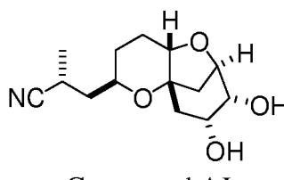
Compound AJ
