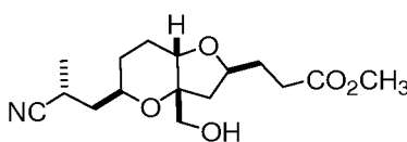
Compound AO
