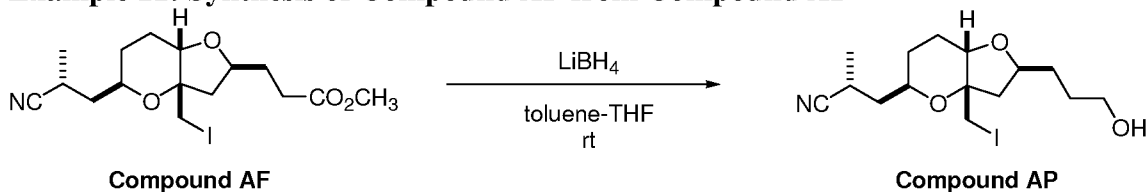
Scheme 21
