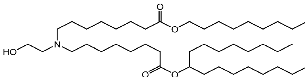
10 (Compound II),
