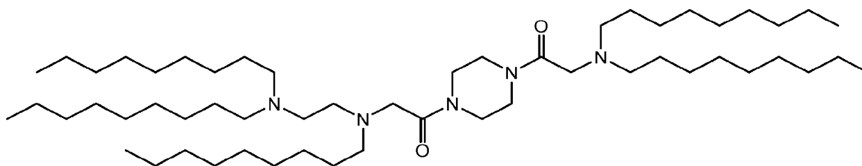
Compound VI
