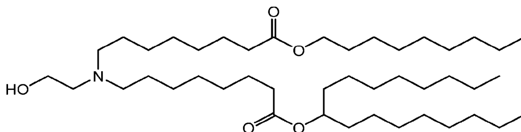
Compound II
