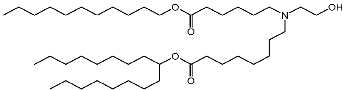
(Compound III),
