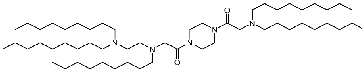
15 (Compound VI),
