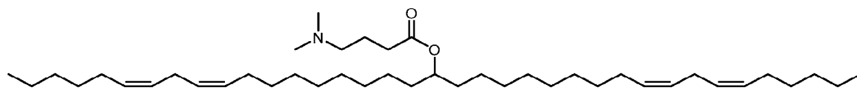
Compound A2
