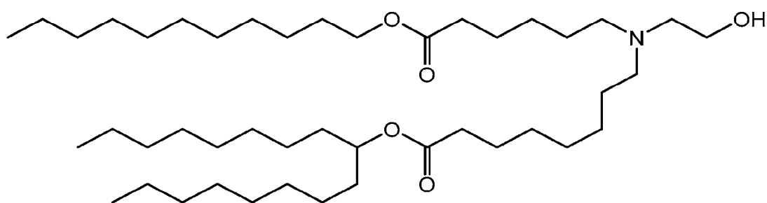
Compound III
