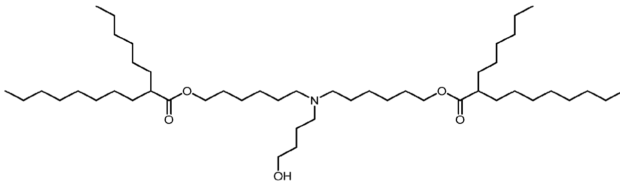
10 Compound A1
