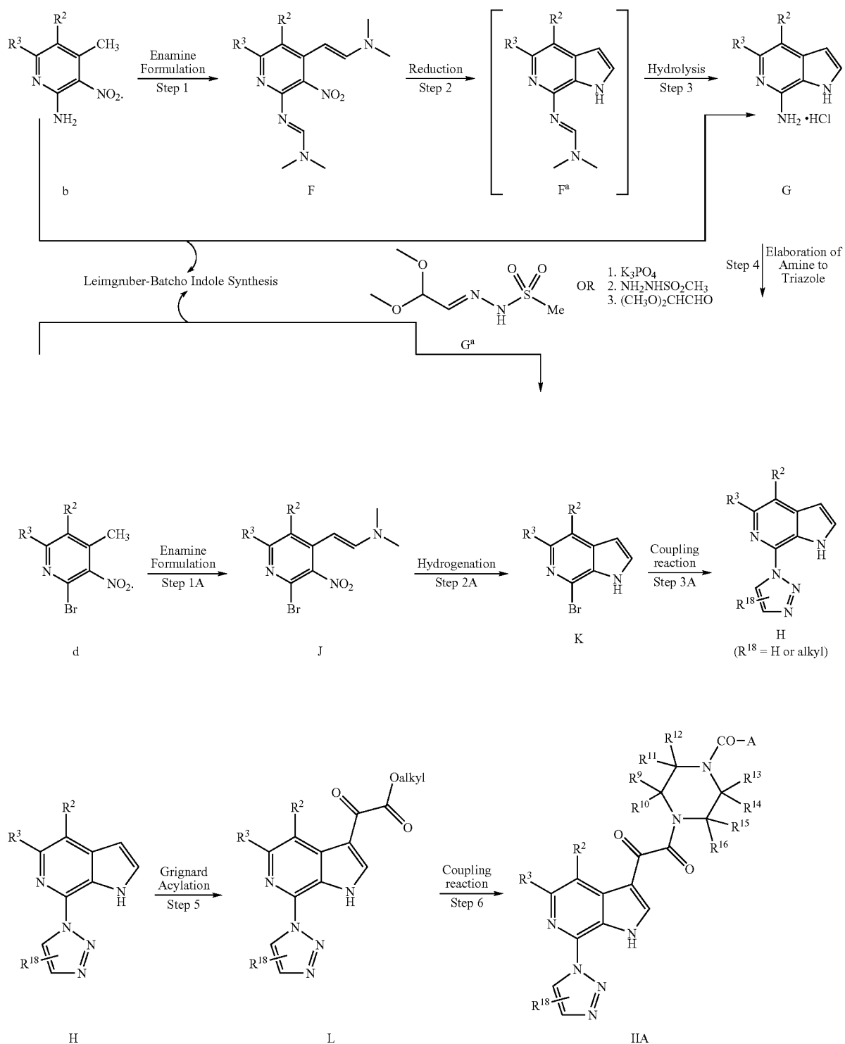
SCHEME II Synthetic route for Compounds II and IIA
