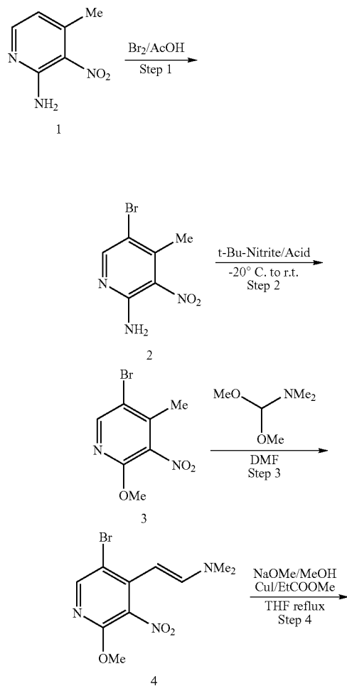
SCHEME IA
