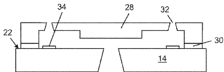
FIG. 2 Prior Art
