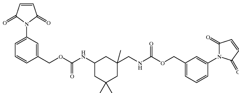
"Bis(m-maleimidobenzyl carbamate) of IPDI"
