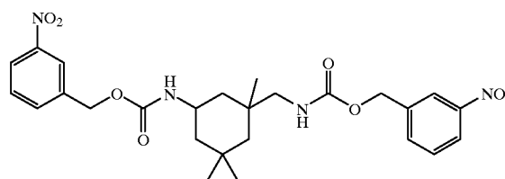
"Bis( m -nitrobenzyl carbamate) of IPDI"
