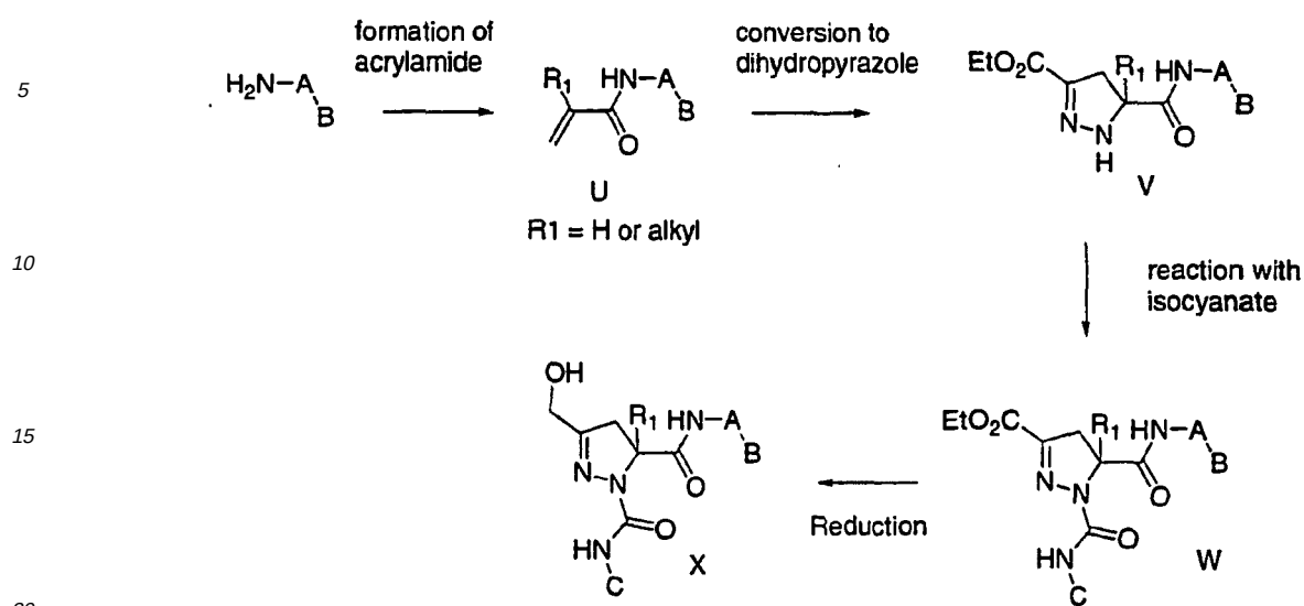
Scheme 5.3
