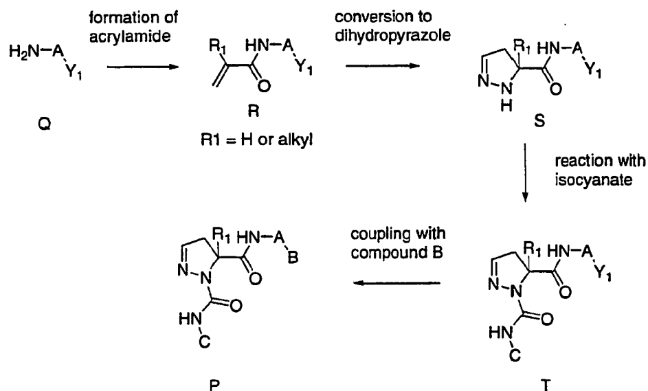
Scheme 5.2
