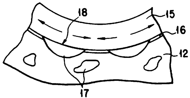
FIG. 4 PRIOR ART
