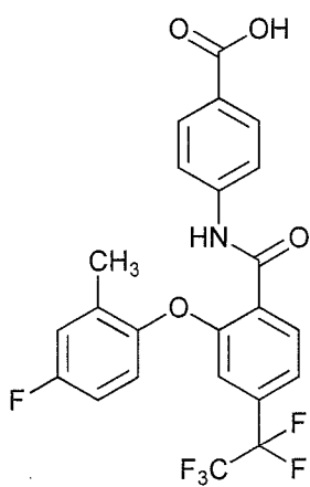
4-(2-(4-fluoro-2-methylphenoxy)-4-(perfluoroethyl)benzamido)benzoic acid;
