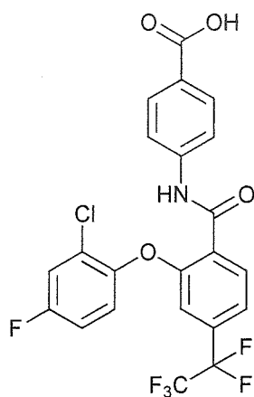
4-(2-(2-chloro-4-fluorophenoxy)-4-(perfluoroethyl)benzamido)benzoic acid;
