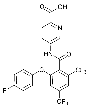
5-(2-(4-fluorophenoxy)-4,6-bis(trifluoromethyl)benzamido)picolinic acid;
