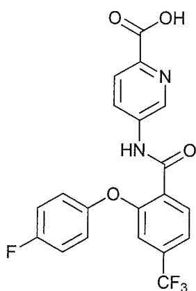
5-(2-(4-fluorophenoxy)-4-(trifluoromethyl)benzamido)picolinic acid;
