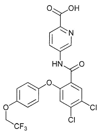
5-(4,5-dichloro-2-(4-(2,2,2-trifluoroethoxy)phenoxy)benzamido)picolinic acid;
