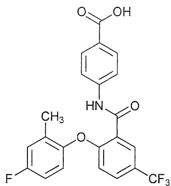
4-(2-(4-fluoro-2-methylphenoxy)-5-(trifluoromethyl)benzamido)benzoic acid;
