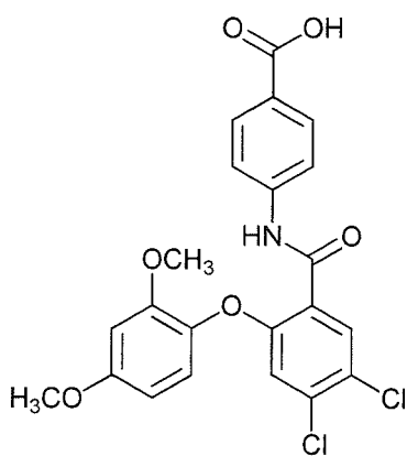
4-(4,5-dichloro-2-(2,4-dimethoxyphenoxy)benzamido)benzoic acid;
