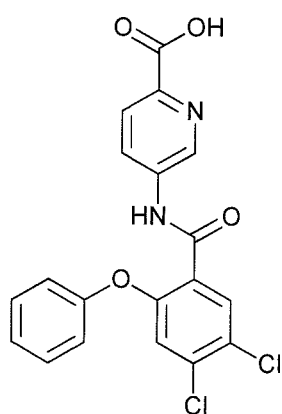
5-(4,5-dichloro-2-phenoxybenzamido)picolinic acid;
