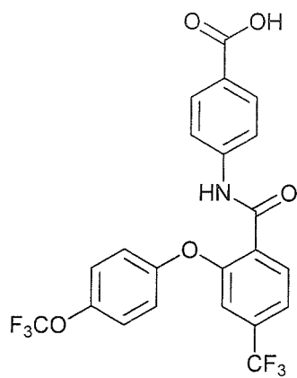
4-(2-(4-(trifluoromethoxy)phenoxy)-4-(trifluoromethyl)benzamido)benzoic acid;
