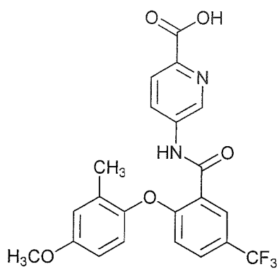
5-(2-(4-methoxy-2-methylphenoxy)-5-(trifluoromethyl)benzamido)picolinic acid;
