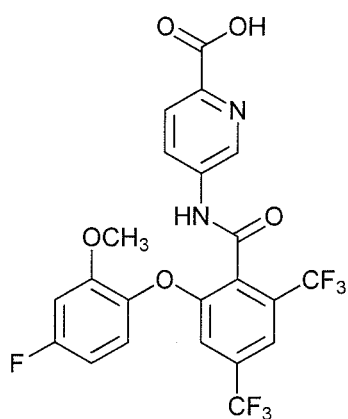
5-(2-(4-fluoro-2-methoxyphenoxy)-4,6-bis(trifluoromethyl)benzamido)picolinic acid;
