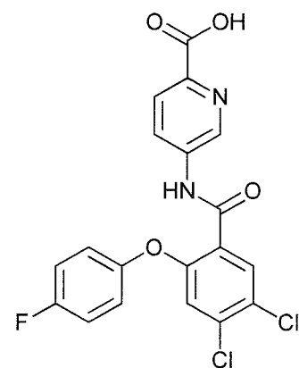
5-(4,5-dichloro-2-(4-fluorophenoxy)benzamido)picolinic acid;
