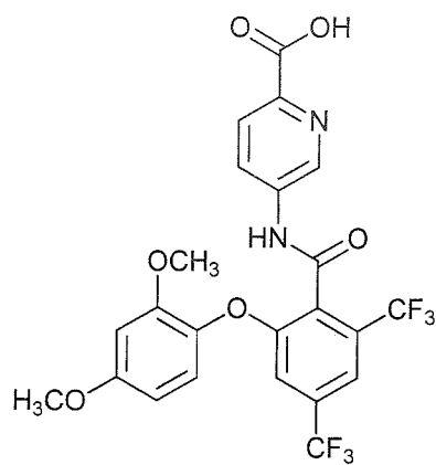
5-(2-(2,4-dimethoxyphenoxy)-4,6-bis(trifluoromethyl)benzamido)picolinic acid;
