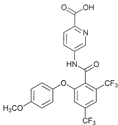
5-(2-(4-methoxyphenoxy)-4,6-bis(trifluoromethyl)benzamido)picolinic acid;
