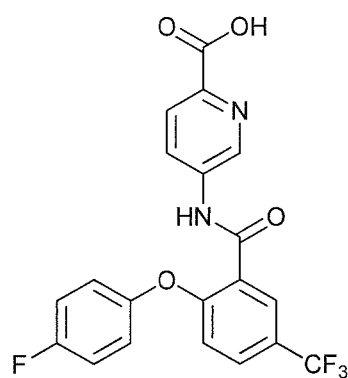
5-(2-(4-fluorophenoxy)-5-(trifluoromethyl)benzamido)picolinic acid;
