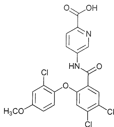
5-(4,5-dichloro-2-(2-chloro-4-methoxyphenoxy)benzamido)picolinic acid;
