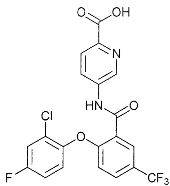
5-(2-(2-chloro-4-fluorophenoxy)-5-(trifluoromethyl)benzamido)picolinic acid;
