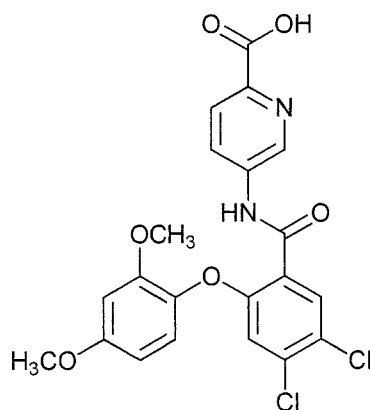
5-(4,5-dichloro-2-(2,4-dimethoxyphenoxy)benzamido)picolinic acid;
