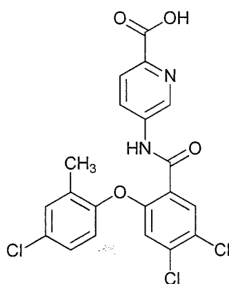
5-(4,5-dichloro-2-(4-chloro-2-methylphenoxy)benzamido)picolinic acid;
