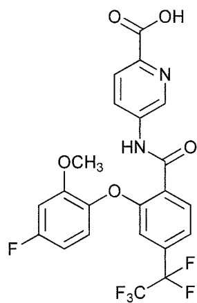
5-(2-(4-fluoro-2-methoxyphenoxy)-4-(perfluoroethyl)benzamido)picolinic acid;
