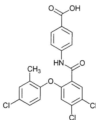
4-(4,5-dichloro-2-(4-chloro-2-methylphenoxy)benzamido)benzoic acid;
