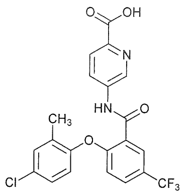
5-(2-(4-chloro-2-methylphenoxy)-5-(trifluoromethyl)benzamido)picolinic acid;
