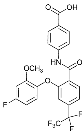
4-(2-(4-fluoro-2-methoxyphenoxy)-4-(perfluoroethyl)benzamido)benzoic acid;
