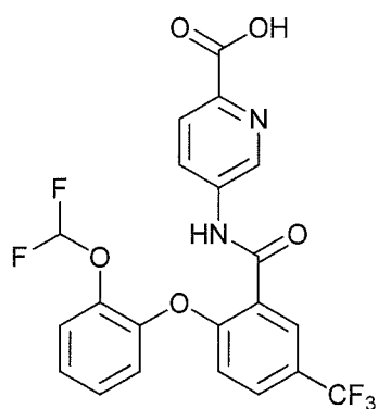
5-(2-(2-(difluoromethoxy)phenoxy)-5-(trifluoromethyl)benzamido)picolinic acid;
