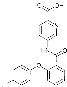
5-(2-(4-fluorophenoxy)benzamido)picolinic acid;
