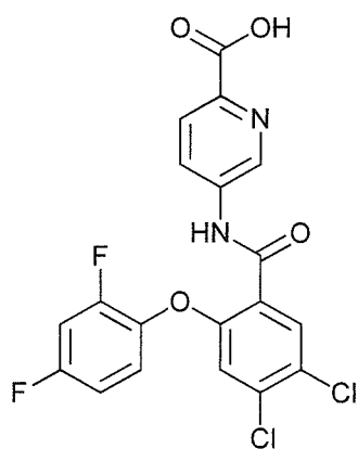
5-(4,5-dichloro-2-(2,4-difluorophenoxy)benzamido)picolinic acid;
