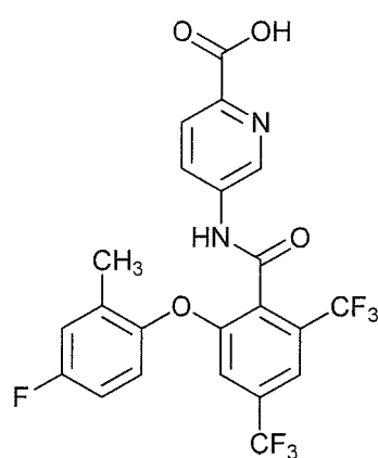
5-(2-(4-fluoro-2-methylphenoxy)-4,6-bis(trifluoromethyl)benzamido)picolinic acid;
