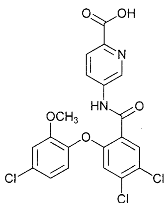
5-(4,5-dichloro-2-(4-chloro-2-methoxyphenoxy)benzamido)picolinic acid;
