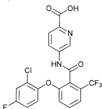
5-(2-(2-chloro-4-fluorophenoxy)-6-(trifluoromethyl)benzamido)picolinic acid;
