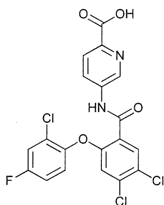
5-(4,5-dichloro-2-(2-chloro-4-fluorophenoxy)benzamido)picolinic acid;
