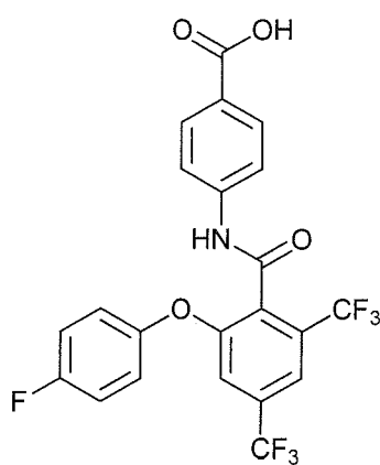
4-(2-(4-fluorophenoxy)-4,6-bis(trifluoromethyl)benzamido)benzoic acid;
