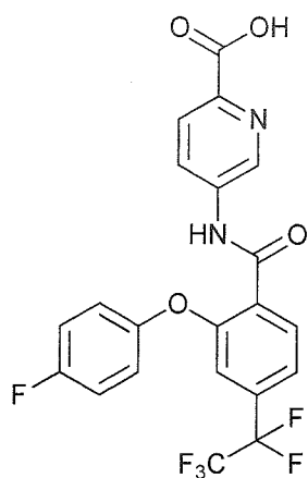
5-(2-(4-fluorophenoxy)-4-(perfluoroethyl)benzamido)picolinic acid;
