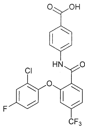
4-(2-(2-chloro-4-fluorophenoxy)-4-(trifluoromethyl)benzamido)benzoic acid;
