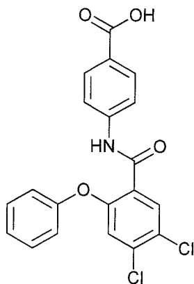
4-(4,5-dichloro-2-phenoxybenzamido)benzoic acid;
