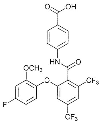
4-(2-(4-fluoro-2-methoxyphenoxy)-4,6-bis(trifluoromethyl)benzamido)benzoic acid;
