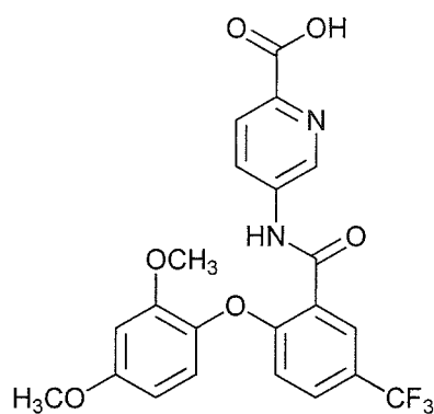
5-(2-(2,4-dimethoxyphenoxy)-5-(trifluoromethyl)benzamido)picolinic acid;
