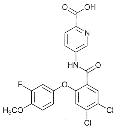
5-(4,5-dichloro-2-(3-fluoro-4-methoxyphenoxy)benzamido)picolinic acid;
