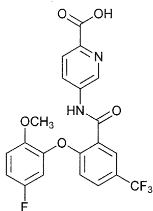
5-(2-(5-fluoro-2-methoxyphenoxy)-5-(trifluoromethyl)benzamido)picolinic acid;
