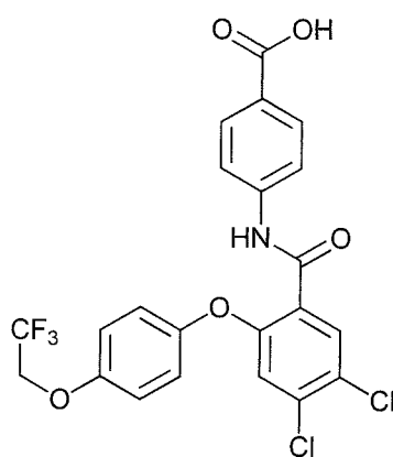
4-(4,5-dichloro-2-(4-(2,2,2-trifluoroethoxy)phenoxy)benzamido)benzoic acid;
