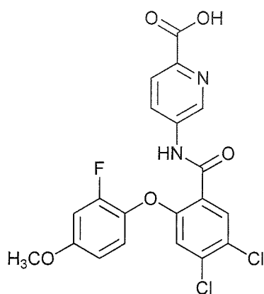
5-(4,5-dichloro-2-(2-fluoro-4-methoxyphenoxy)benzamido)picolinic acid;
