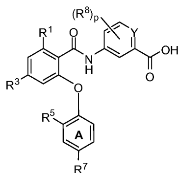
I'-H
