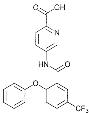
5-(2-phenoxy-5-(trifluoromethyl)benzamido)picolinic acid;
