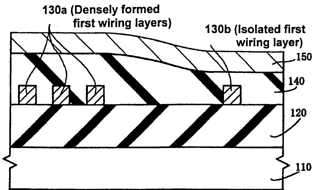
Fig. 18 (Prior Art)
