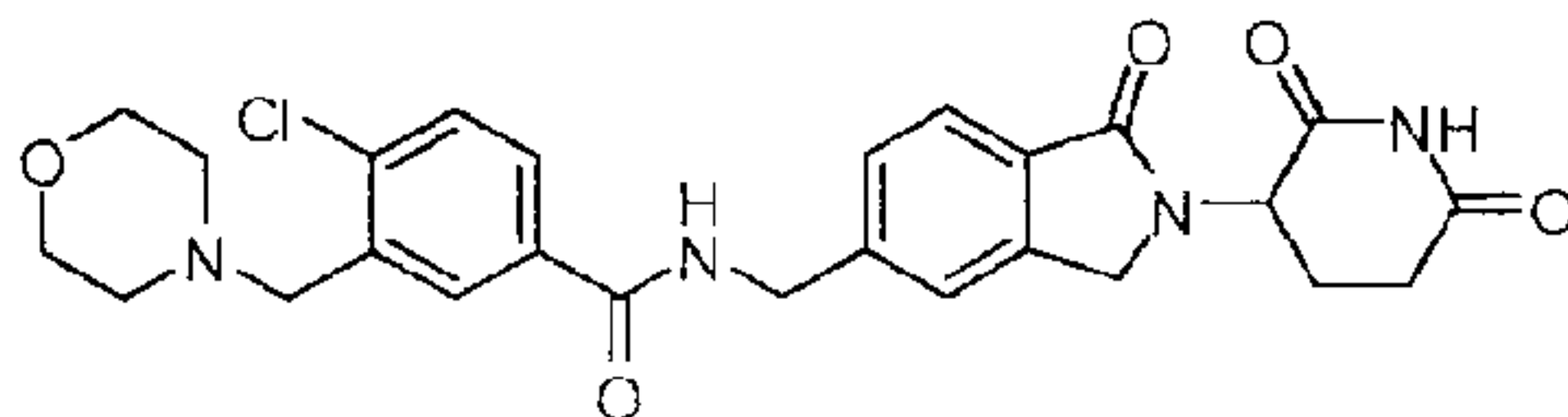
4-chloro-N-((2-(2,6-dioxopiperidin-3-yl)-1-oxoisindolin-5-yl)methyl)-3-(morpholinomethyl)benzamide;
