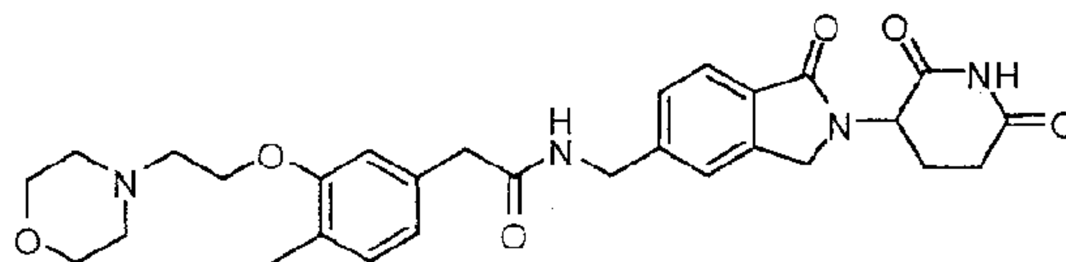
N-((2-(2,6-dioxopiperidin-3-yl)-1-oxoisindolin-5-yl)methyl)-2-(4-methyl-3-(2-morpholinoethoxy)phenyl)acetamide;
