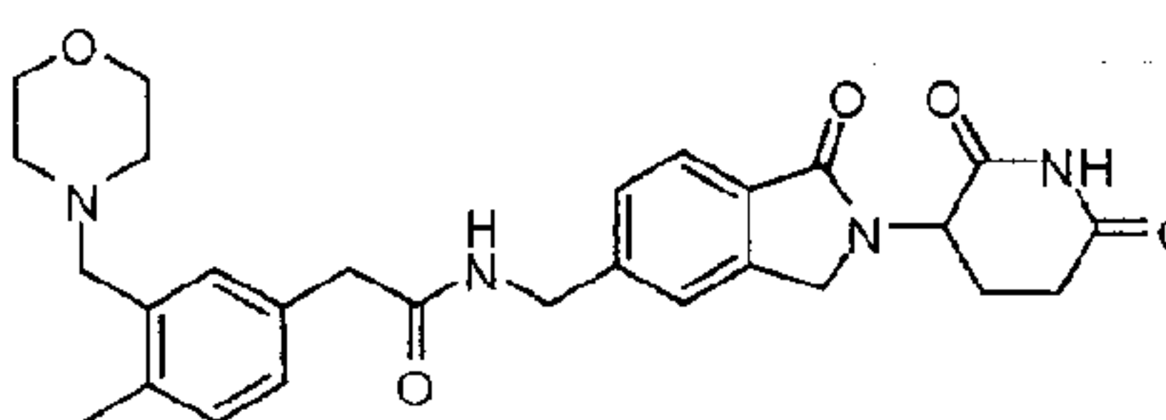
N-((2-(2,6-dioxopiperidin-3-yl)-1-oxoisindolin-5-yl)methyl)-2-(4-methyl-3-(morpholinomethyl)phenyl)acetamide;
