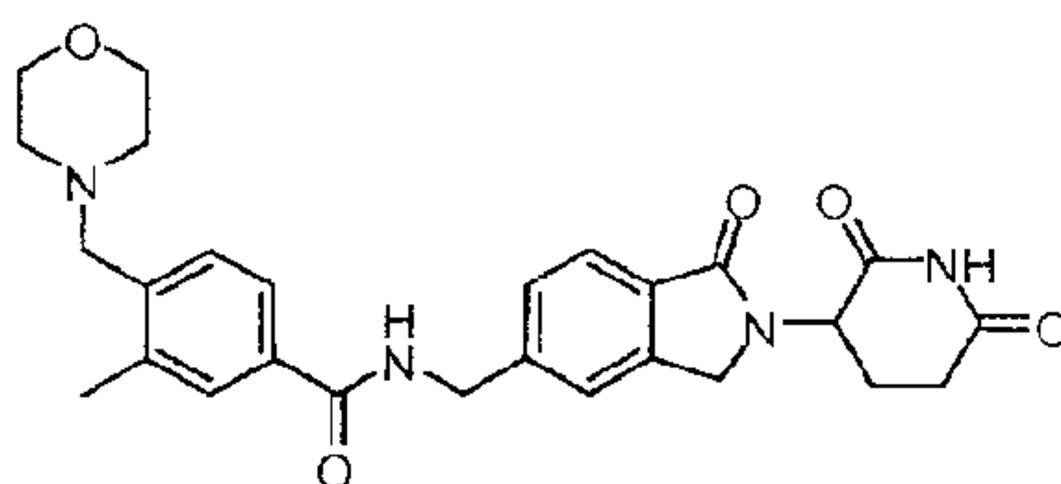
N-((2-(2,6-dioxopiperidin-3-yl)-1-oxoisindolin-5-yl)methyl)-3-methyl-4-(morpholinomethyl)benzamide;
