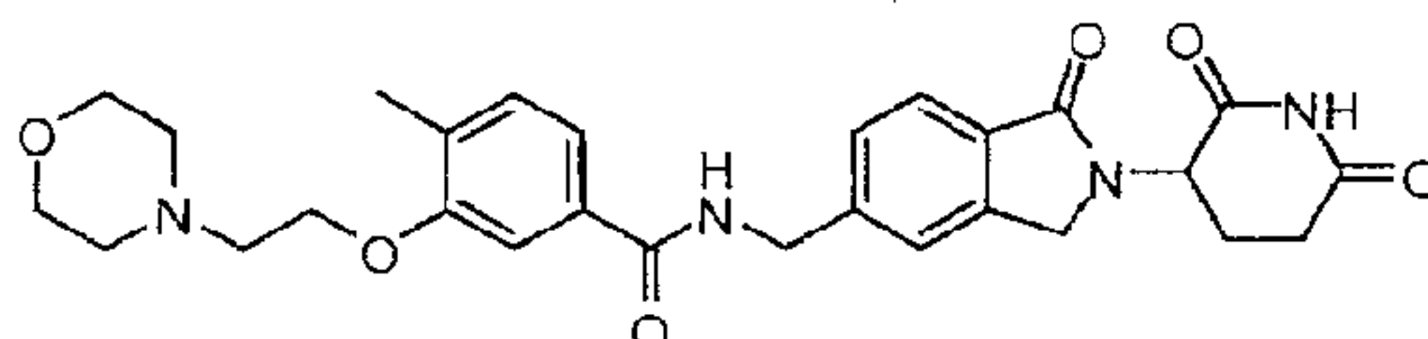
N-((2-(2,6-dioxopiperidin-3-yl)-1-oxoisindolin-5-yl)methyl)-4-methyl-3-(2-morpholinoethoxy)benzamide; and
