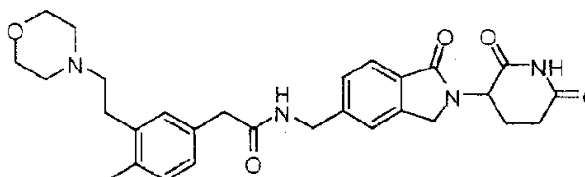
N-((2-(2,6-dioxopiperidin-3-yl)-1-oxoisindolin-5-yl)methyl)-2-(4-methyl-3-(2-morpholinoethyl)phenyl)acetamide;
