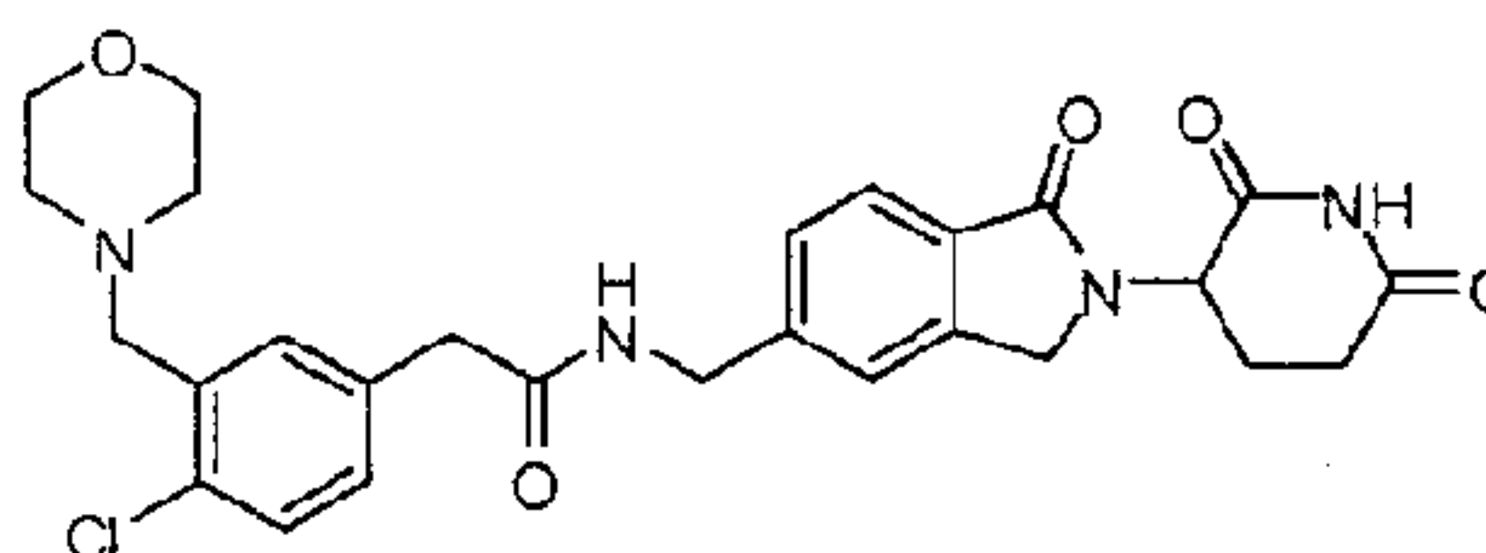
2-(4-chloro-3-(morpholinomethyl)phenyl)-N-((2-(2,6-dioxopiperidin-3-yl)-1-oxoisindolin-5-yl)methyl)acetamide;
