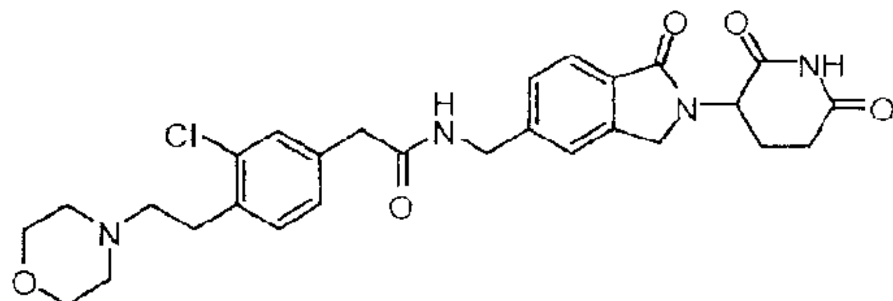
2-(3-chloro-4-(2-morpholinoethyl)phenyl)-N-((2-(2,6-dioxopiperidin-3-yl)-1-oxoisindolin-5-yl)methyl)acetamide;
