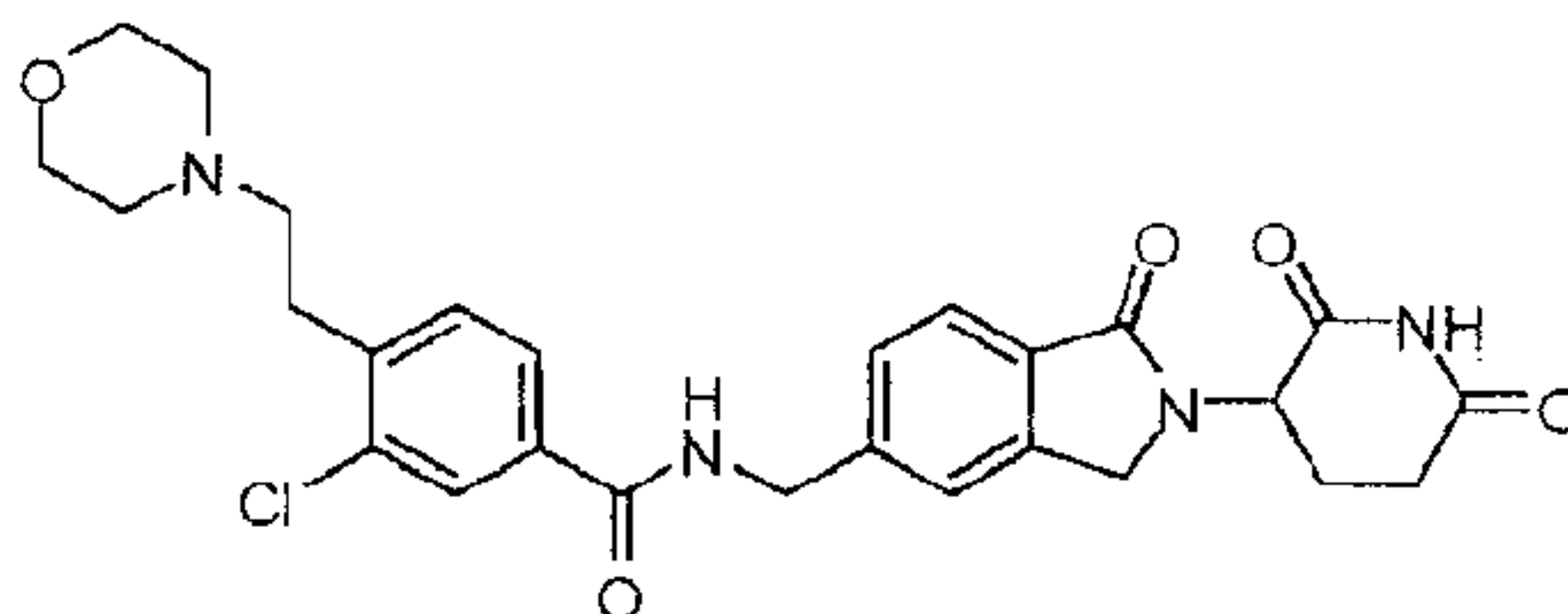
3-chloro-N-((2-(2,6-dioxopiperidin-3-yl)-1-oxoisindolin-5-yl)methyl)-4-(2-morpholinoethyl)benzamide;
