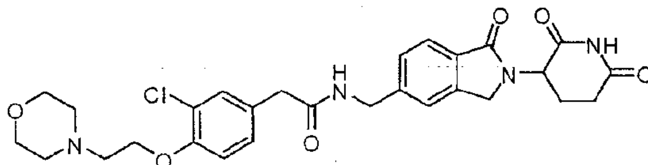
2-(3-chloro-4-(2-morpholinoethoxy)phenyl)-N-((2-(2,6-dioxopiperidin-3-yl)-1-oxoisindolin-5-yl)methyl)acetamide;
