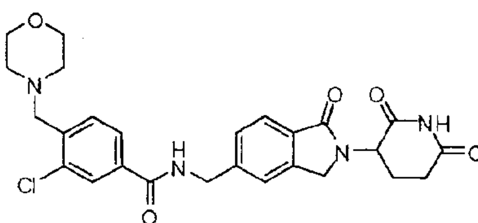
3-chloro-N-((2-(2,6-dioxopiperidin-3-yl)-1-oxoisindolin-5-yl)methyl)-4-(morpholinomethyl)benzamide;
