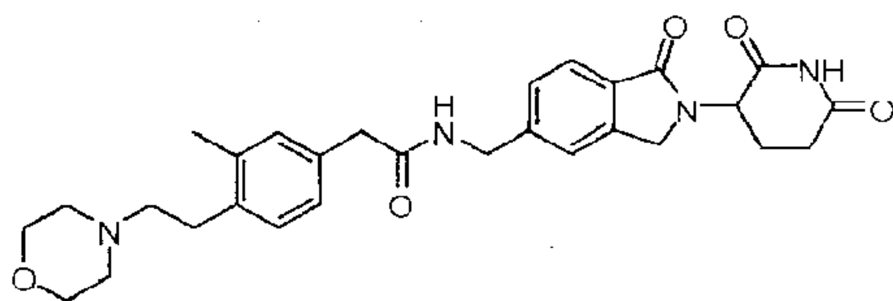
N-((2-(2,6-dioxopiperidin-3-yl)-1-oxoisindolin-5-yl)methyl)-2-(3-methyl-4-(2-morpholinoethyl)phenyl)acetamide;
