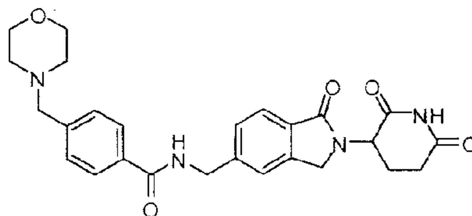
N-((2-(2,6-dioxopiperidin-3-yl)-1-oxoisindolin-5-yl)methyl)-4-(morpholinomethyl)benzamide;
