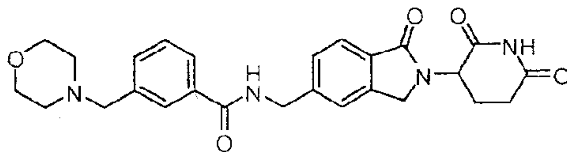
N-((2-(2,6-dioxopiperidin-3-yl)-1-oxoisindolin-5-yl)methyl)-3-(morpholinomethyl)benzamide;
