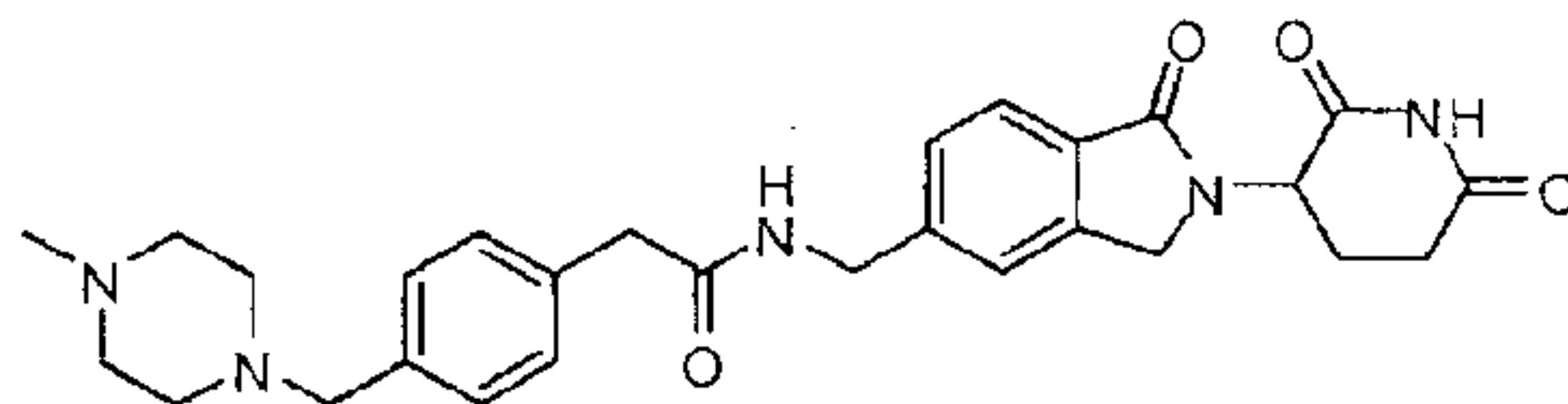
N-((2-(2,6-dioxopiperidin-3-yl)-1-oxoisindolin-5-yl)methyl)-2-(4-((4-methylpiperazin-1-yl)methyl)phenyl)acetamide;
