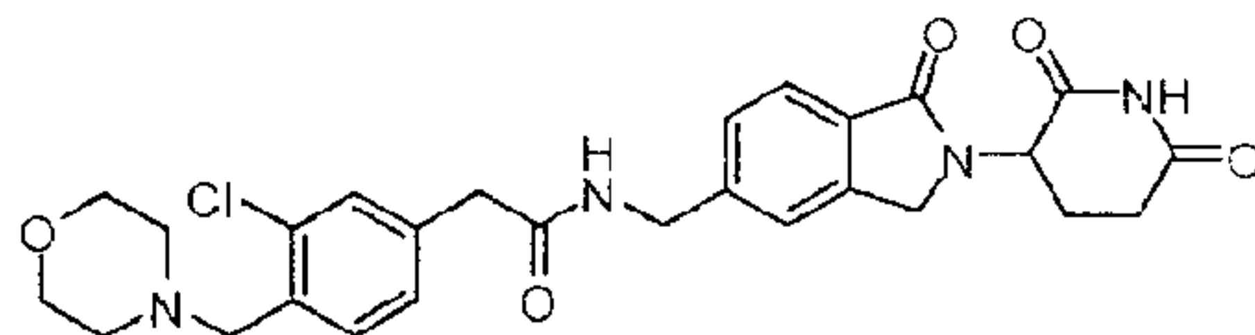
2-(3-chloro-4-(morpholinomethyl)phenyl)-N-((2-(2,6-dioxopiperidin-3-yl)-1-oxoisindolin-5-yl)methyl)acetamide;
