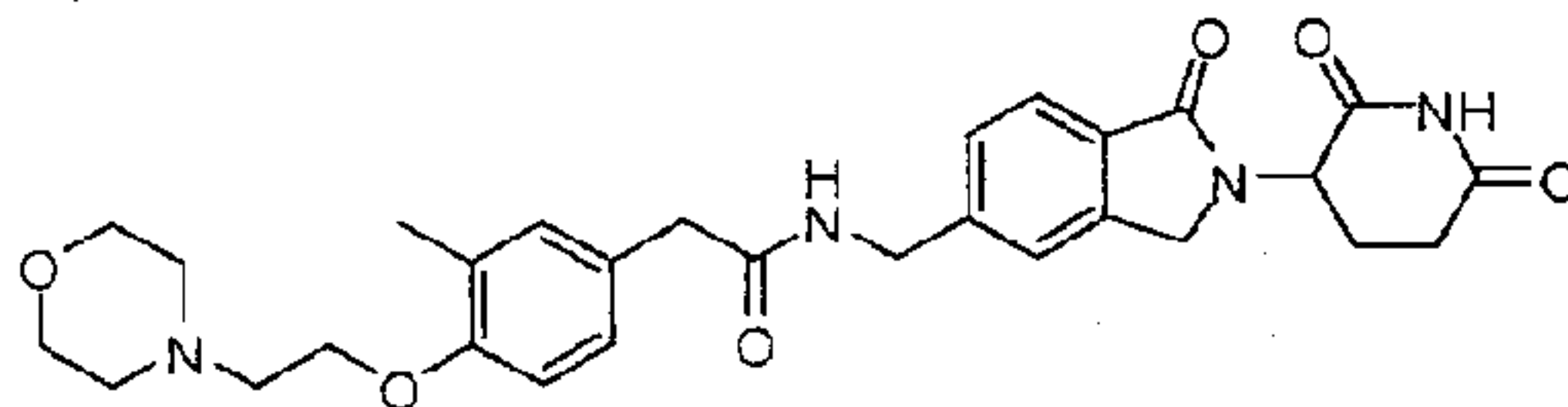
N-((2-(2,6-dioxopiperidin-3-yl)-1-oxoisindolin-5-yl)methyl)-2-(3-methyl-4-(2-morpholinoethoxy)phenyl)acetamide;
