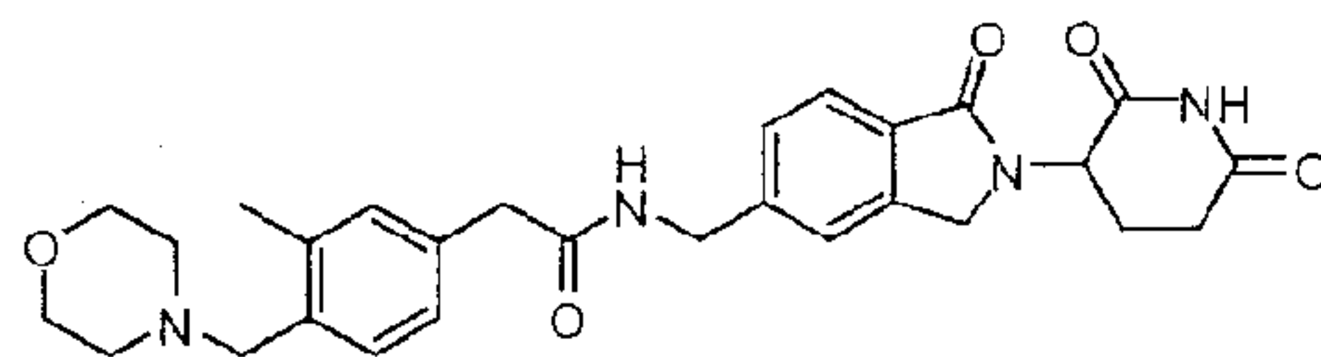
N-((2-(2,6-dioxopiperidin-3-yl)-1-oxoisindolin-5-yl)methyl)-2-(3-methyl-4-(morpholinomethyl)phenyl)acetamide;
