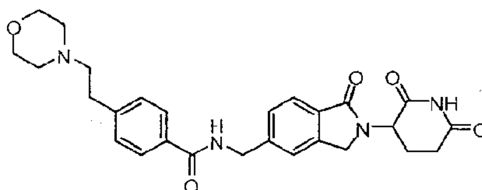
N-((2-(2,6-dioxopiperidin-3-yl)-1-oxoisindolin-5-yl)methyl)-4-(2-morpholinoethyl)benzamide;
