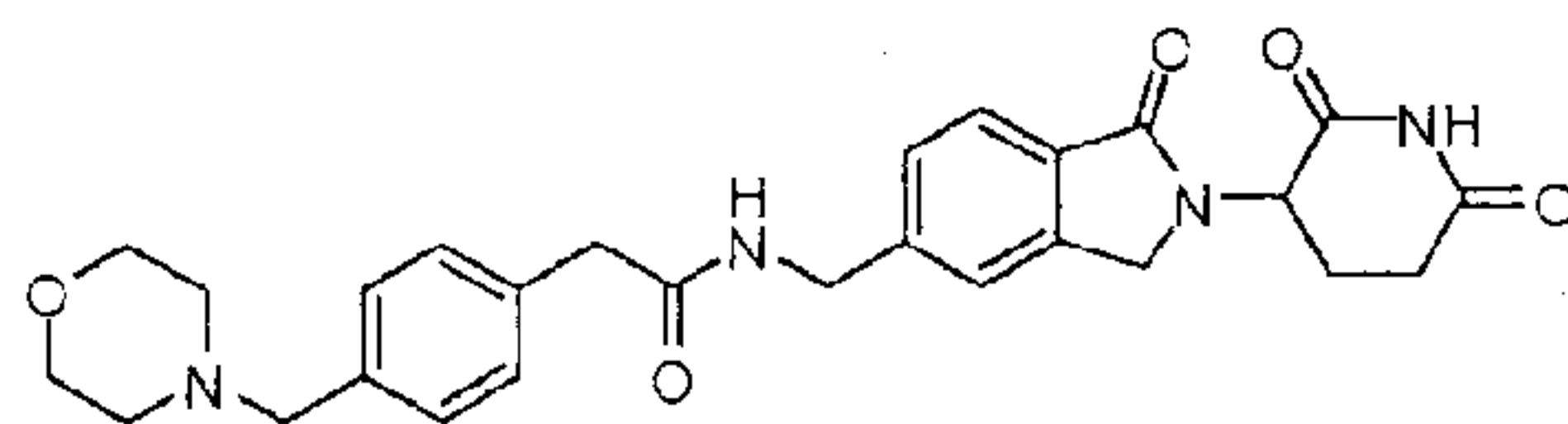
N-((2-(2,6-dioxopiperidin-3-yl)-1-oxoisindolin-5-yl)methyl)-2-(4-(morpholinomethyl)phenyl)acetamide;
