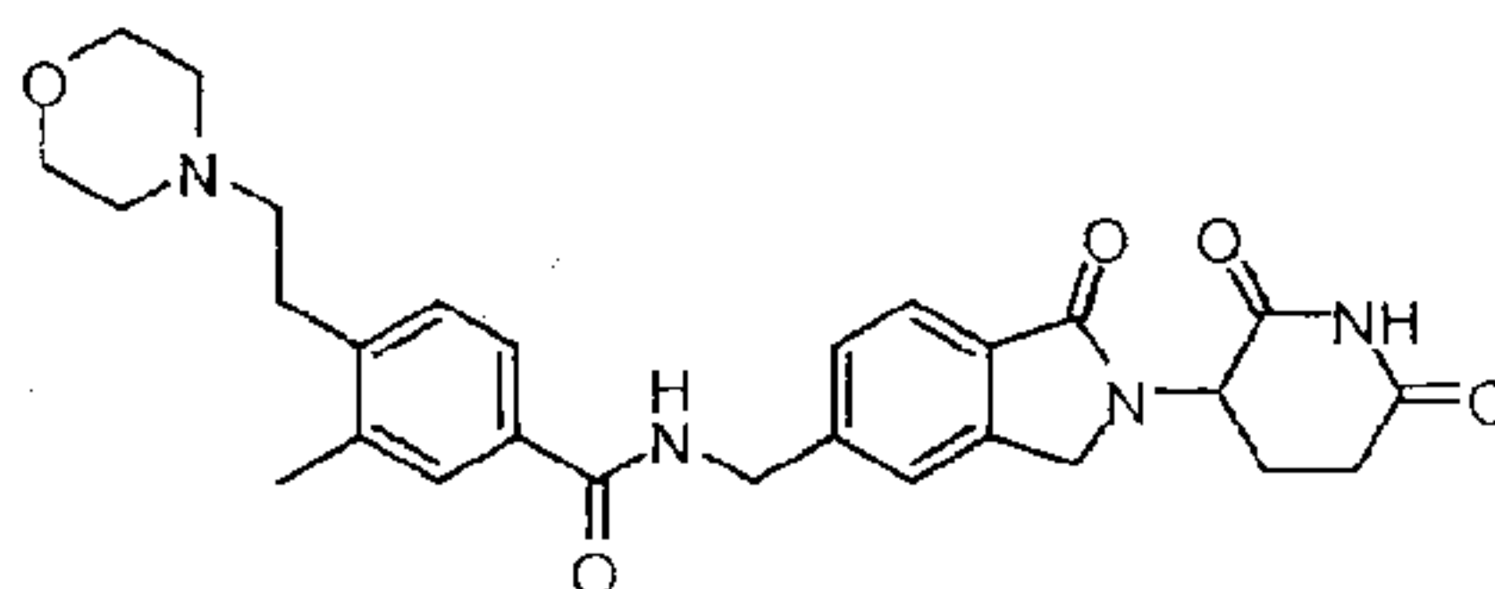
N-((2-(2,6-dioxopiperidin-3-yl)-1-oxoisindolin-5-yl)methyl)-3-methyl-4-(2-morpholinoethyl)benzamide;
