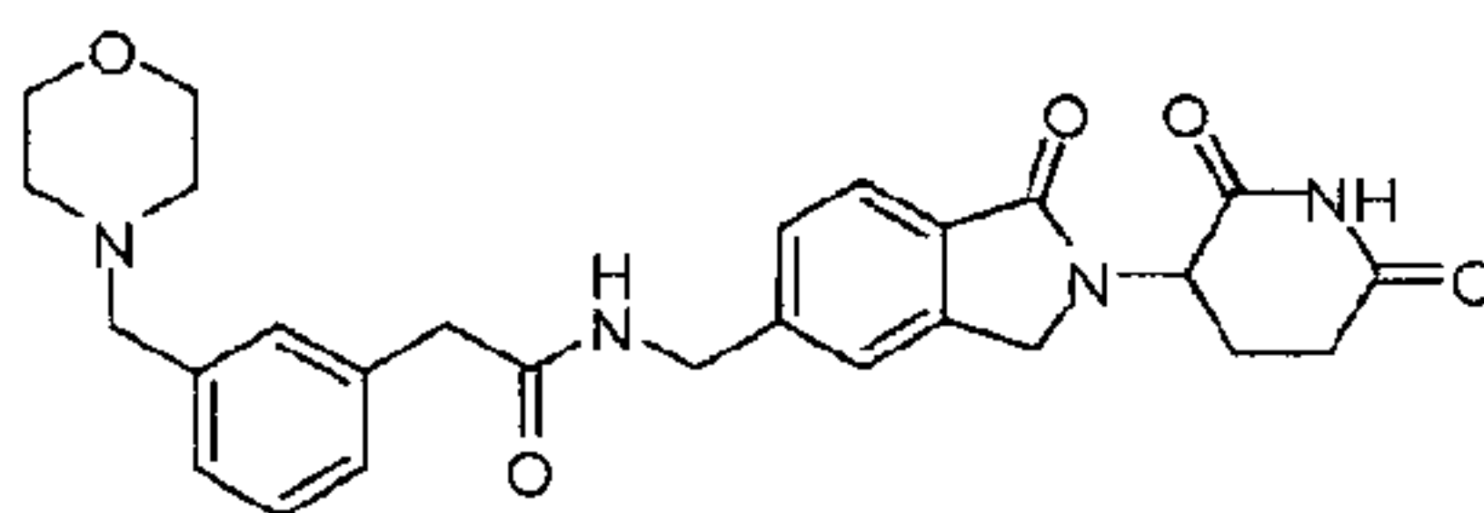
N-((2-(2,6-dioxopiperidin-3-yl)-1-oxoisindolin-5-yl)methyl)-2-(3-(morpholinomethyl)phenyl)acetamide;
