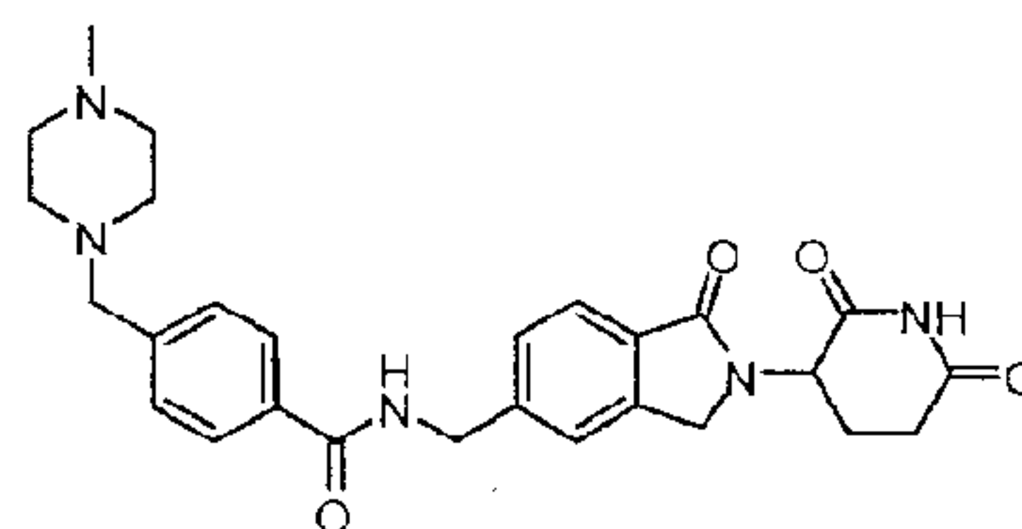
N-((2-(2,6-dioxopiperidin-3-yl)-1-oxoisindolin-5-yl)methyl)-4-((4-methylpiperazin-1-yl)methyl)benzamide;
