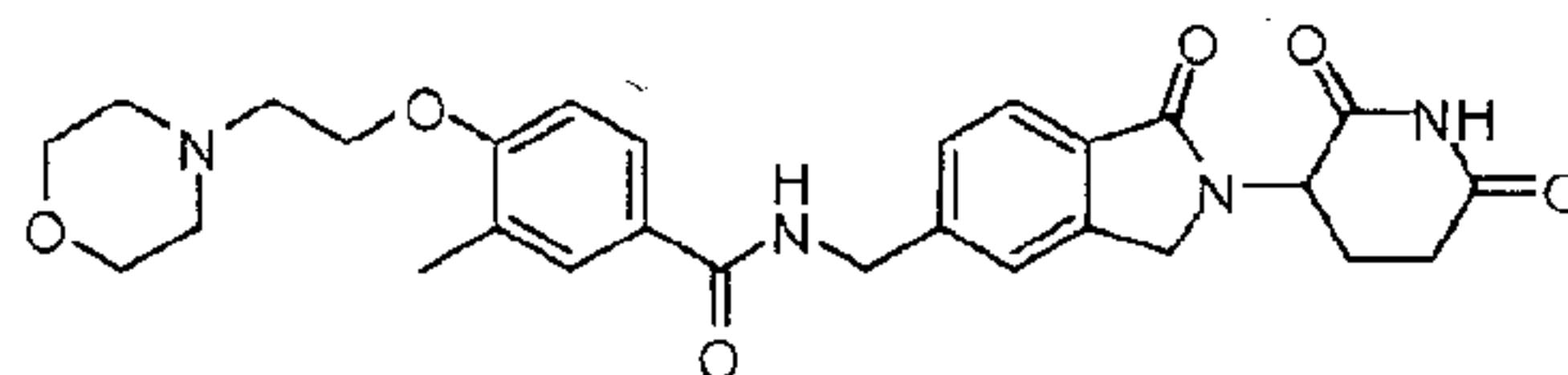
N-((2-(2,6-dioxopiperidin-3-yl)-1-oxoisindolin-5-yl)methyl)-3-methyl-4-(2-morpholinoethoxy)benzamide;
