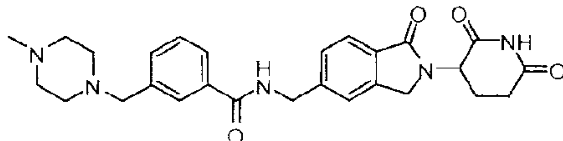
N-((2-(2,6-dioxopiperidin-3-yl)-1-oxoisindolin-5-yl)methyl)-3-((4-methylpiperazin-1-yl)methyl)benzamide;
