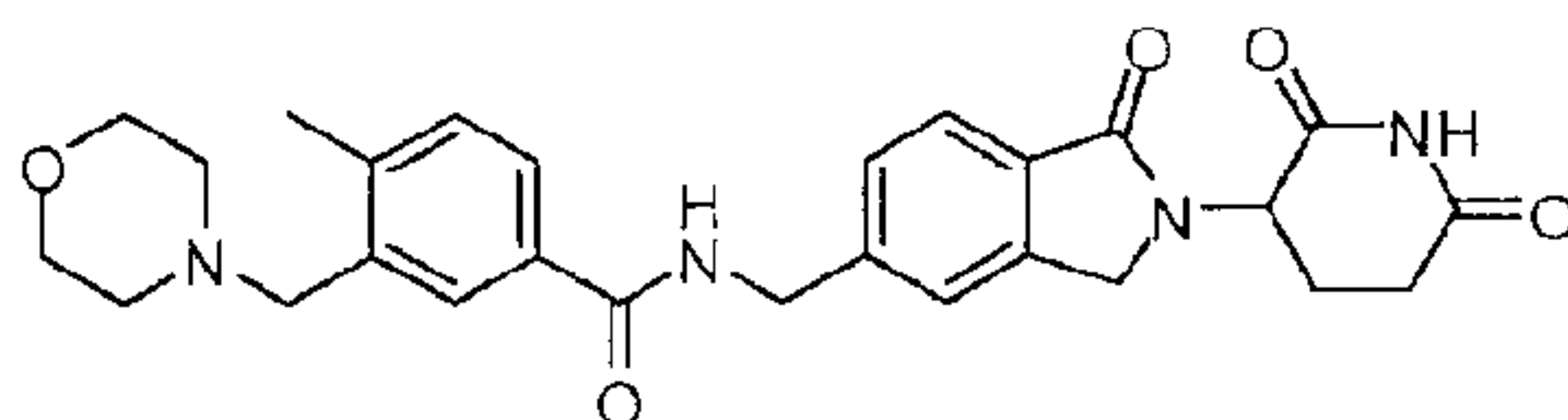
N-((2-(2,6-dioxopiperidin-3-yl)-1-oxoisindolin-5-yl)methyl)-4-methyl-3-(morpholinomethyl)benzamide;
