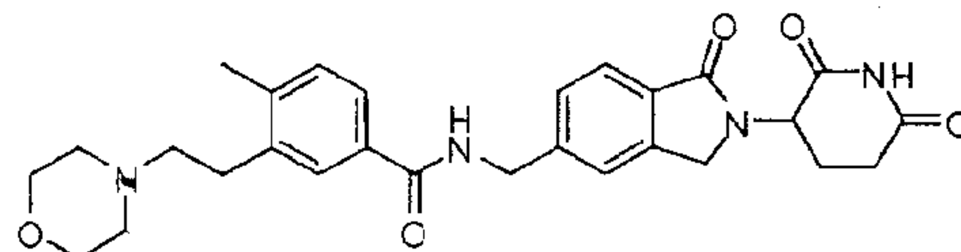
N-((2-(2,6-dioxopiperidin-3-yl)-1-oxoisindolin-5-yl)methyl)-4-methyl-3-(2-morpholinoethyl)benzamide;
