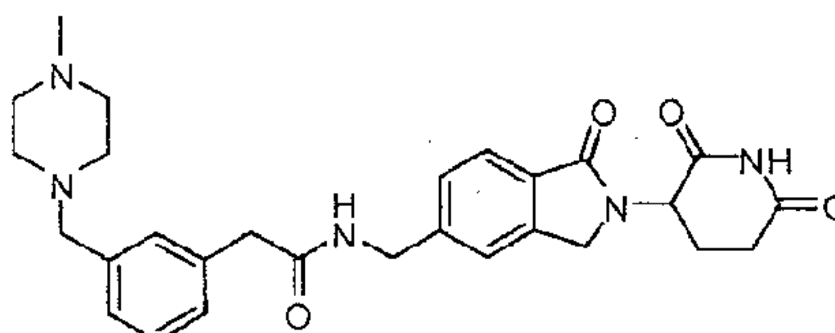
N-((2-(2,6-dioxopiperidin-3-yl)-1-oxoisindolin-5-yl)methyl)-2-(3-((4-methylpiperazin-1-yl)methyl)phenyl)acetamide;
