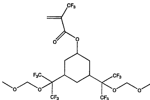
TFMA-3,5-HFA-CHOH-MOM
