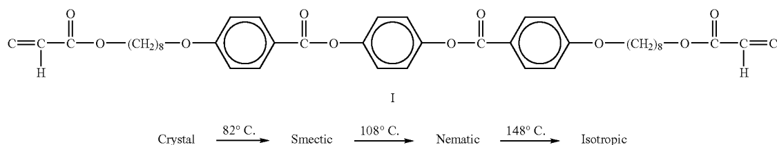
Formula 3: Liquid crystalline diacrylate
