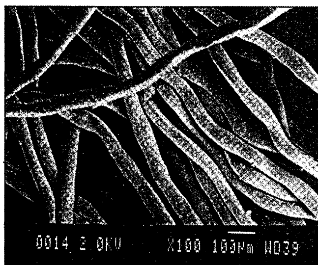
FIG. 4 CROSSLINKED FIBER
