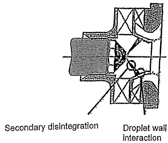
Fig. 1: Prefilming atomizer according to Joos et al. (1993)
