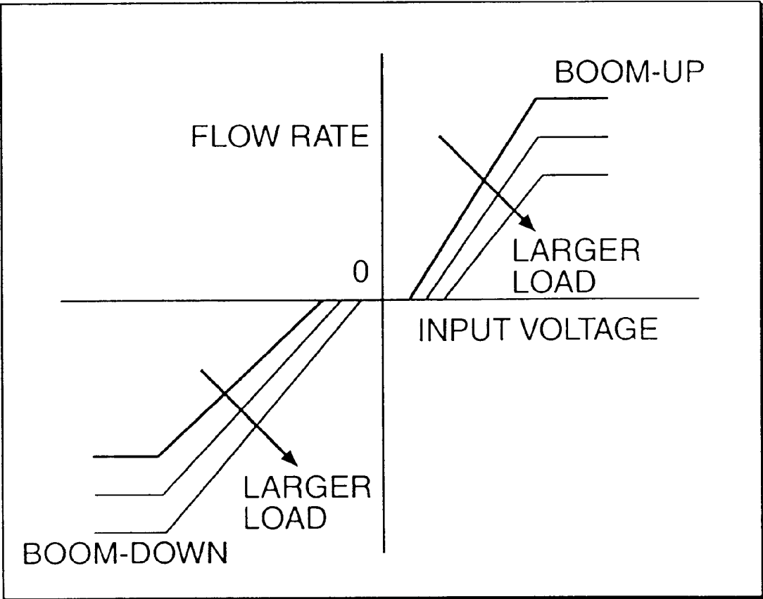
FLOW RATE CHARACTERISTIC
