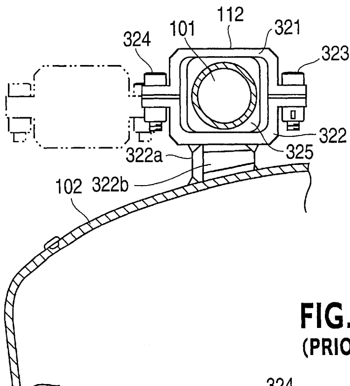
FIG. 8(a) (PRIOR ART)
