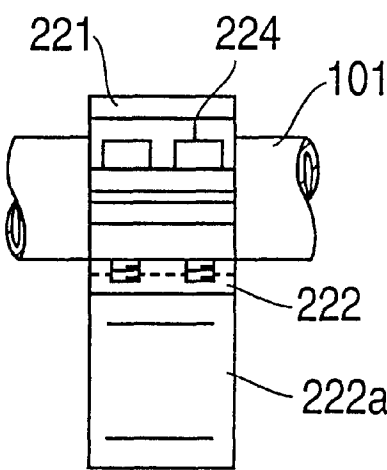
FIG. 7(c) (PRIOR ART)
