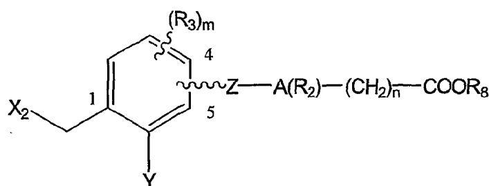
21 Formula 6
