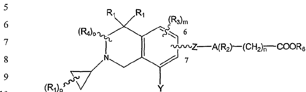
11 Formula 3
