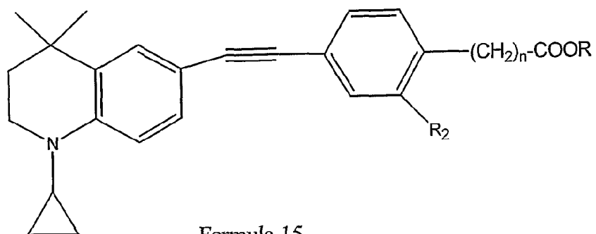
Formula 15
