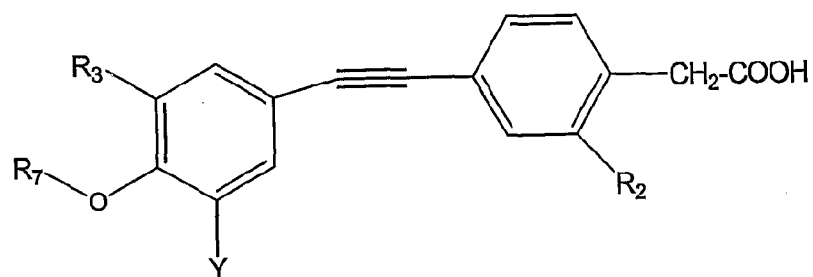
Formula 13
