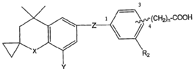
Formula 9
