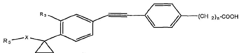
Formula 10
