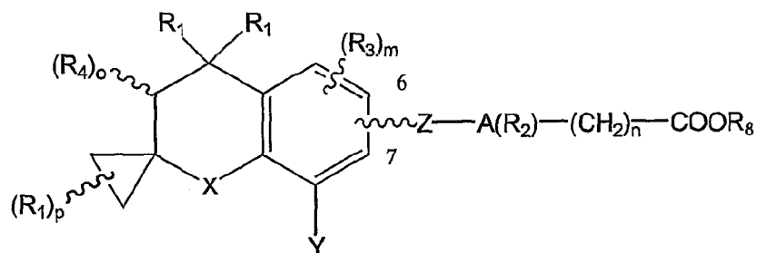
Formula 1
