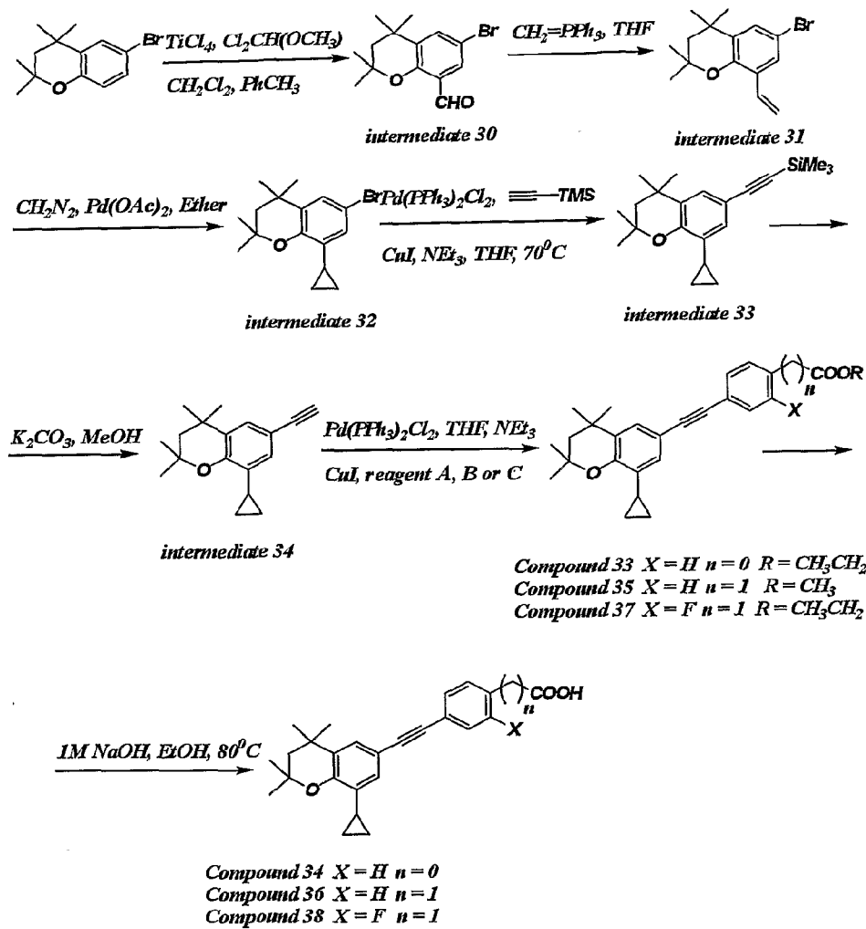
REACTION SCHEME 6
