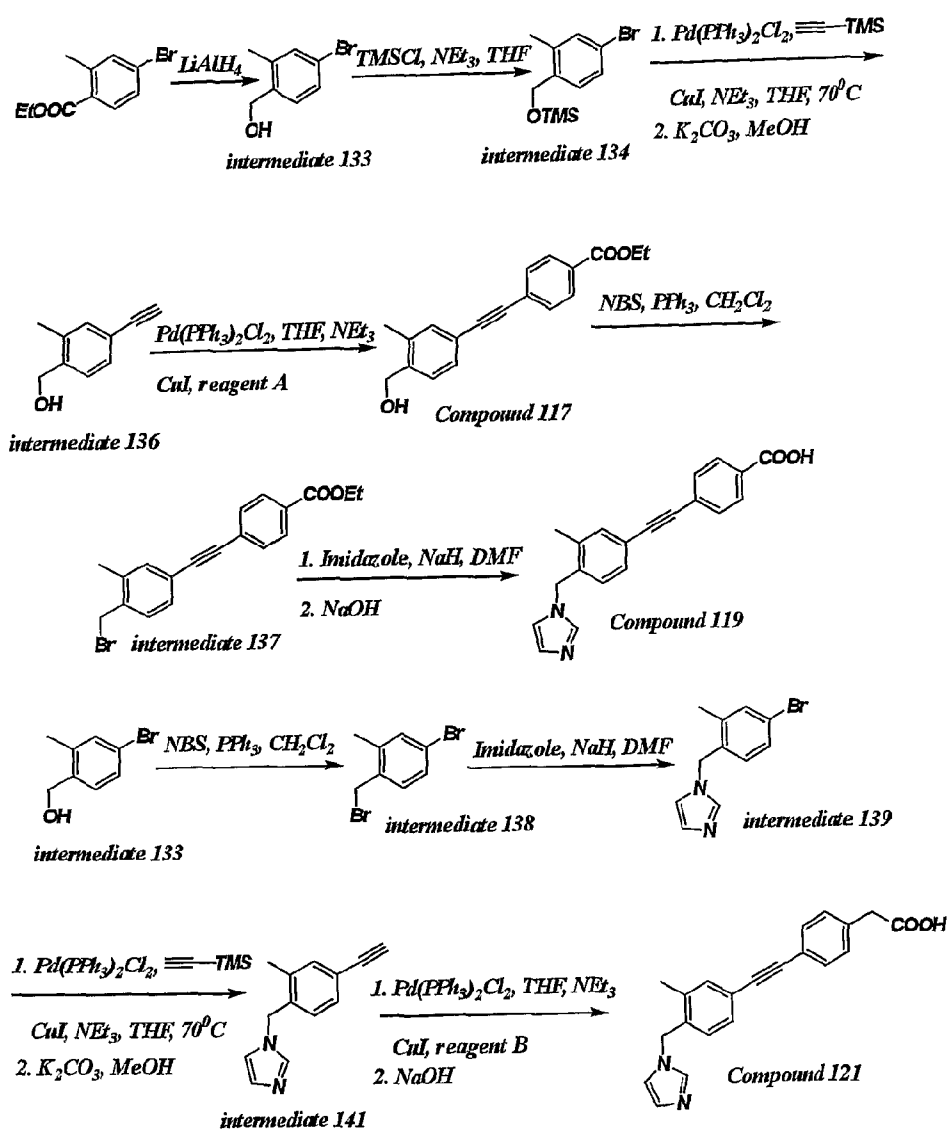
REACTION SCHEME 13
