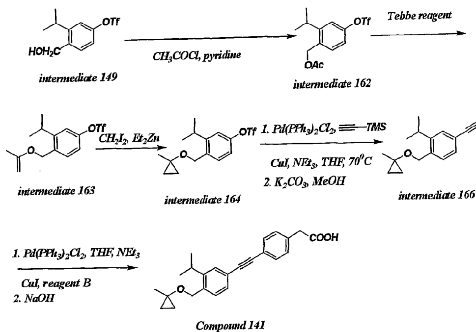
REACTION SCHEME 17
