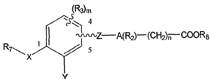
Formula 5
