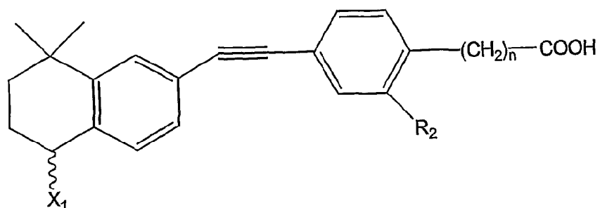
Formula 12
