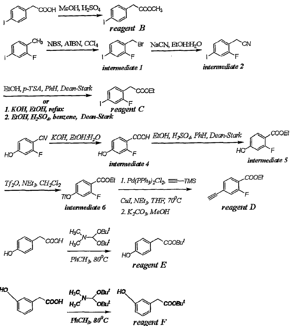
REACTION SCHEME 1
