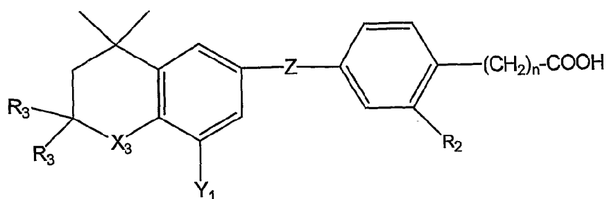
Formula 16
