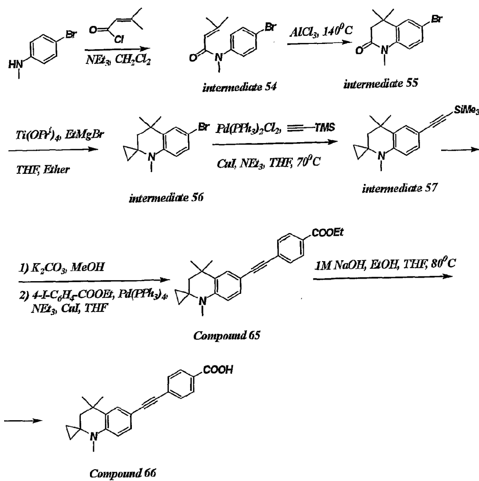
REACTION SCHEME 9
