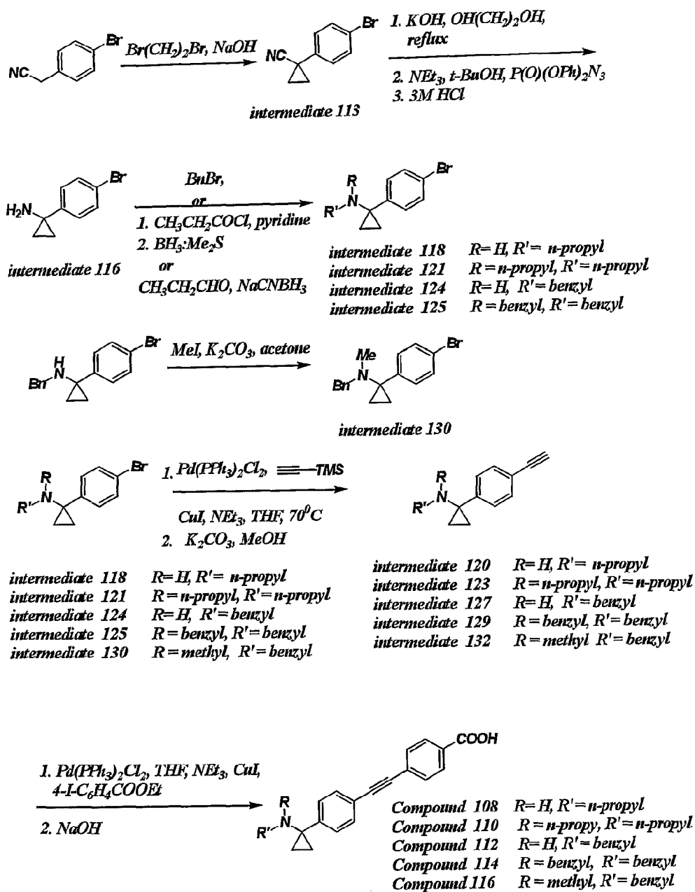
REACTION SCHEME 12
