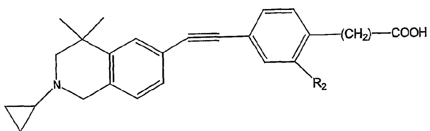
Formula 11
