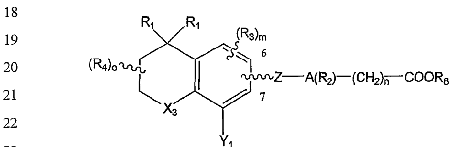
24 Formula 8
