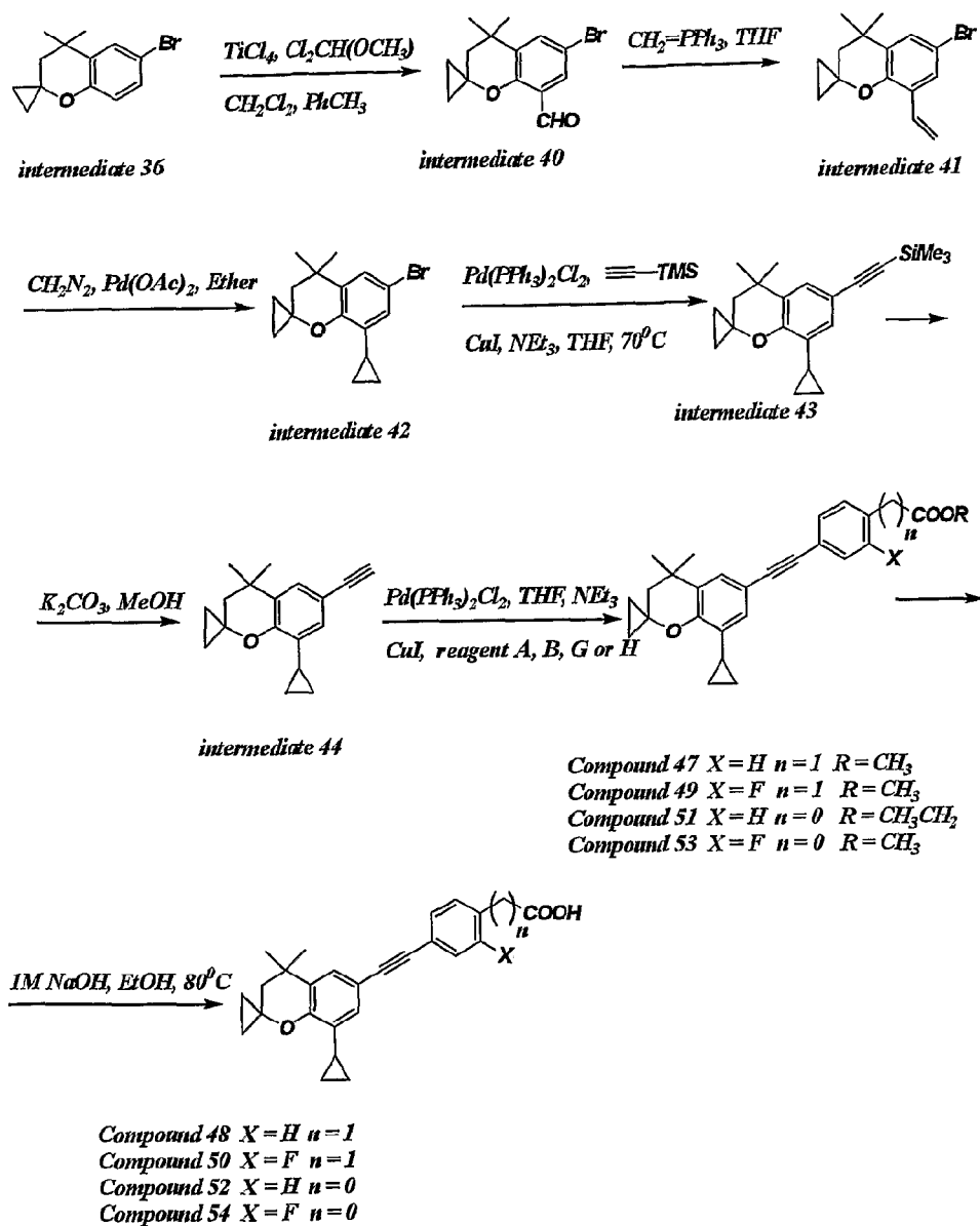
REACTION SCHEME 8
