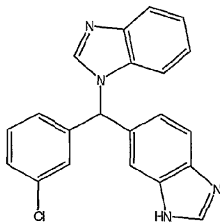
LIARAZOLE
