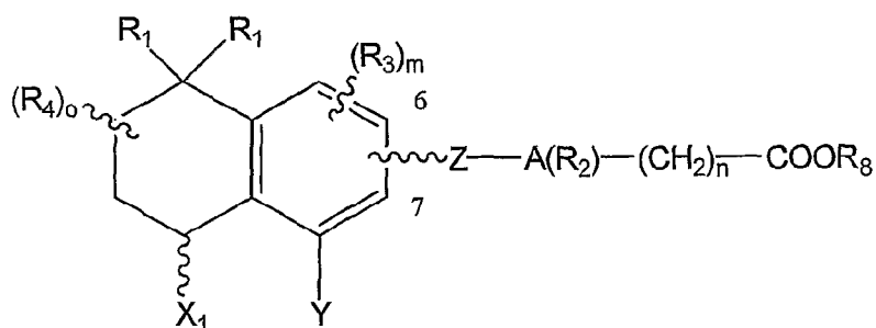
Formula 4
