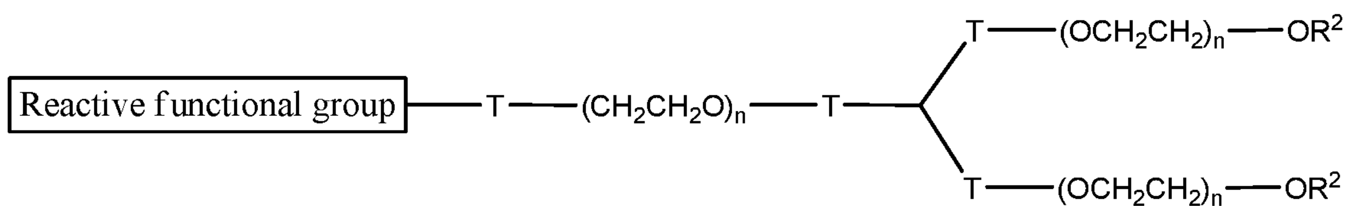
Formula D
