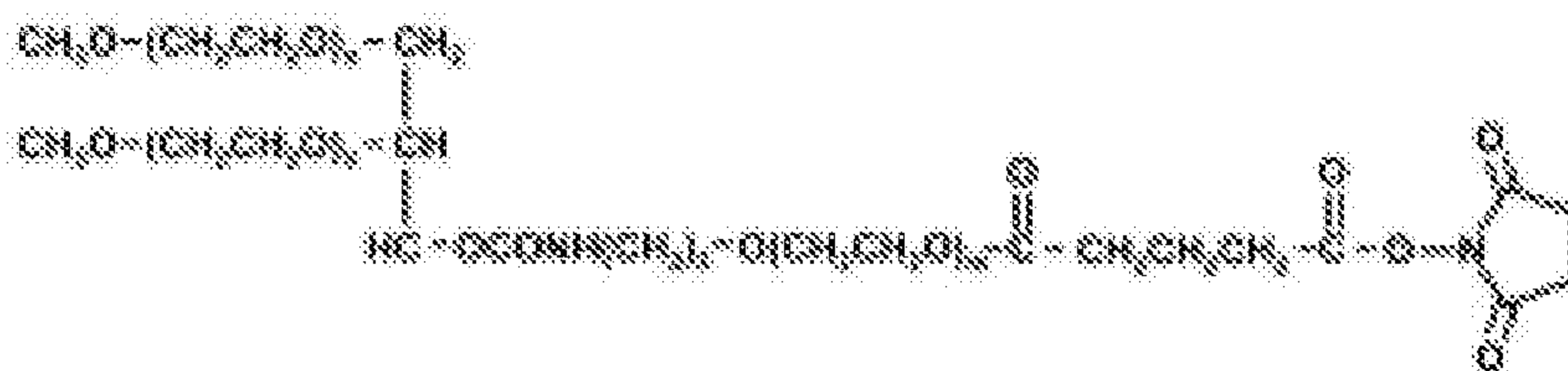
Formula XII
