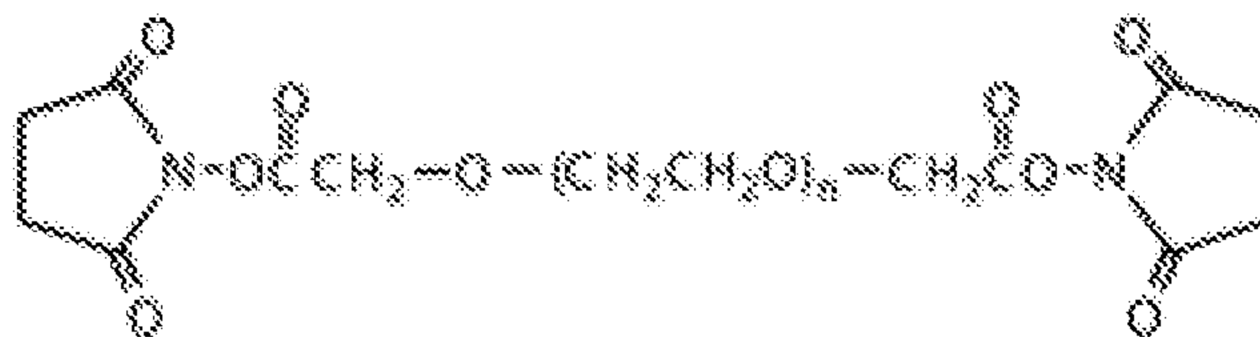
Formula IV
