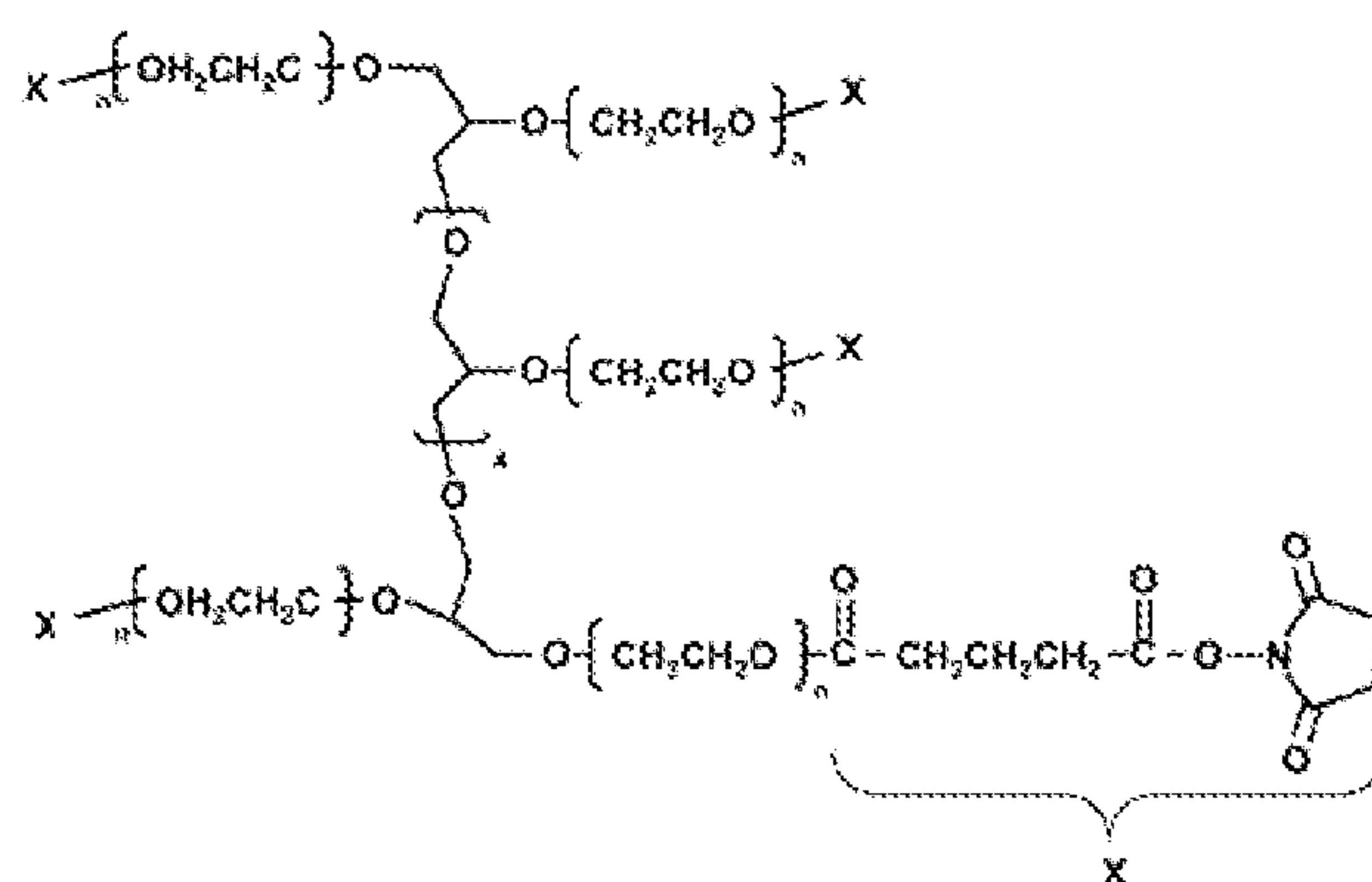
Formula VI
