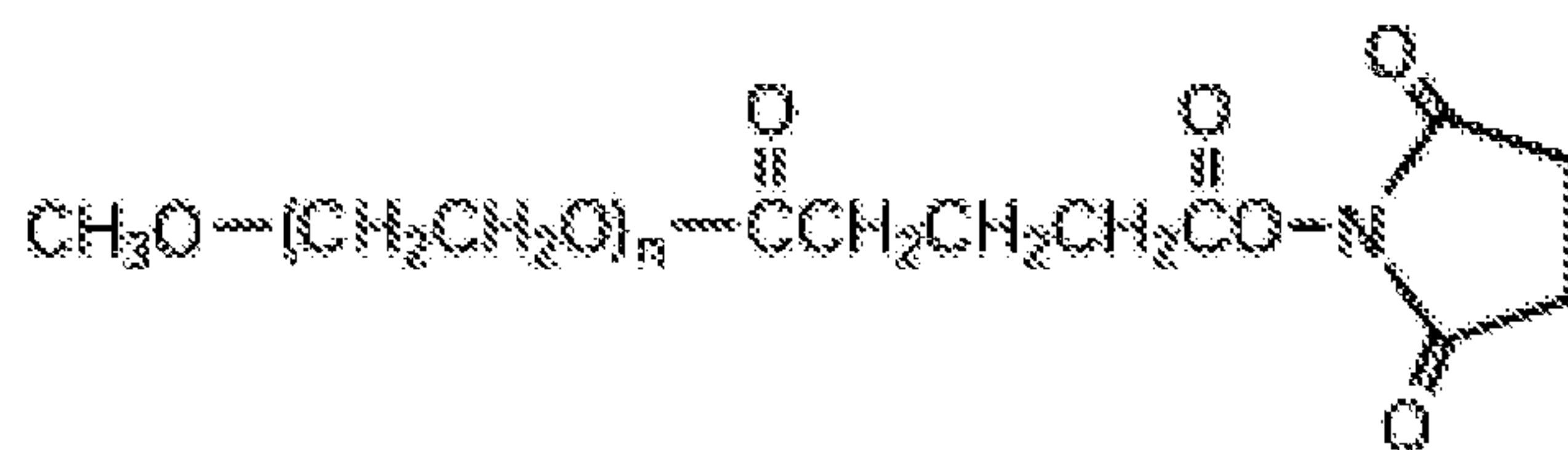
Formula Ia.
