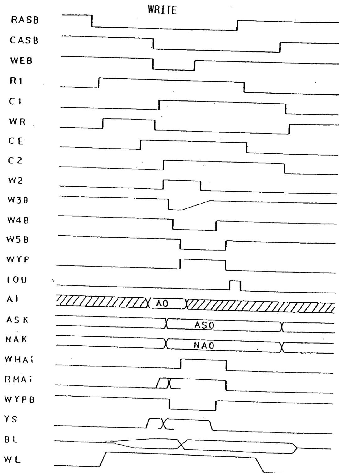
FIG. 76 CAS SYSTEM (WRITE OPERATION)
