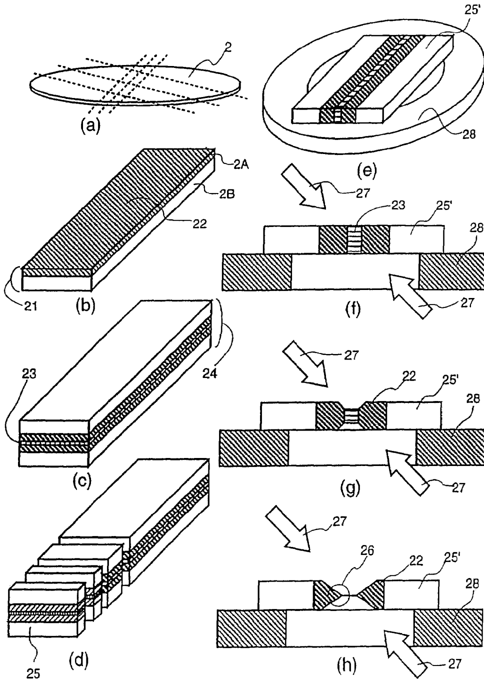
FIG.2 (PRIOR ART)
