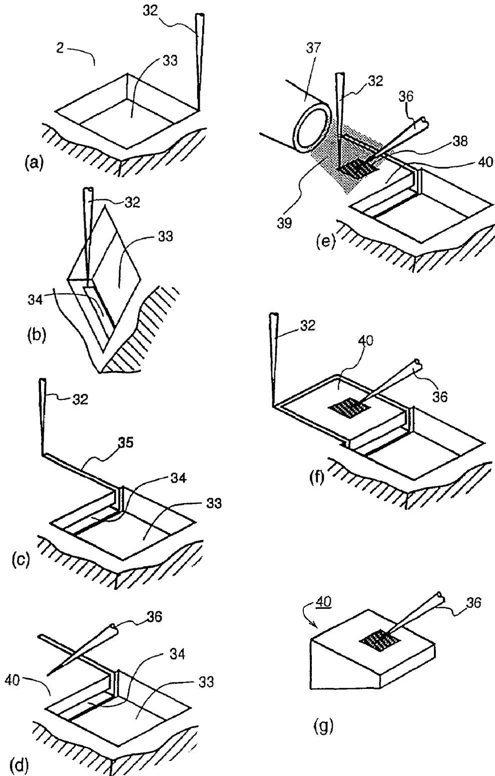
FIG. 4 (PRIOR ART)
