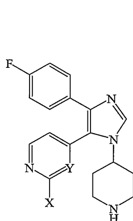
P6 X = H, Y = CH; HEP 689 (SB 235699)
