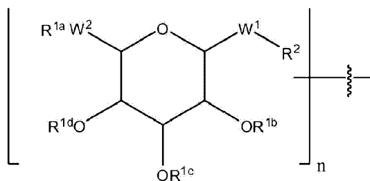
Formula 2-I
