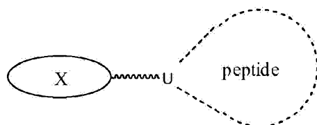
Formula 2-I-A
