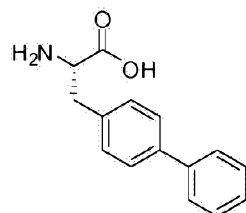
2-L-biphenyl-alanine (Bip)
