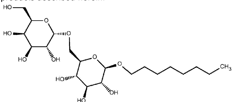
1-Octyl beta-D-melibioside
