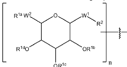
Formula 2-I-A
